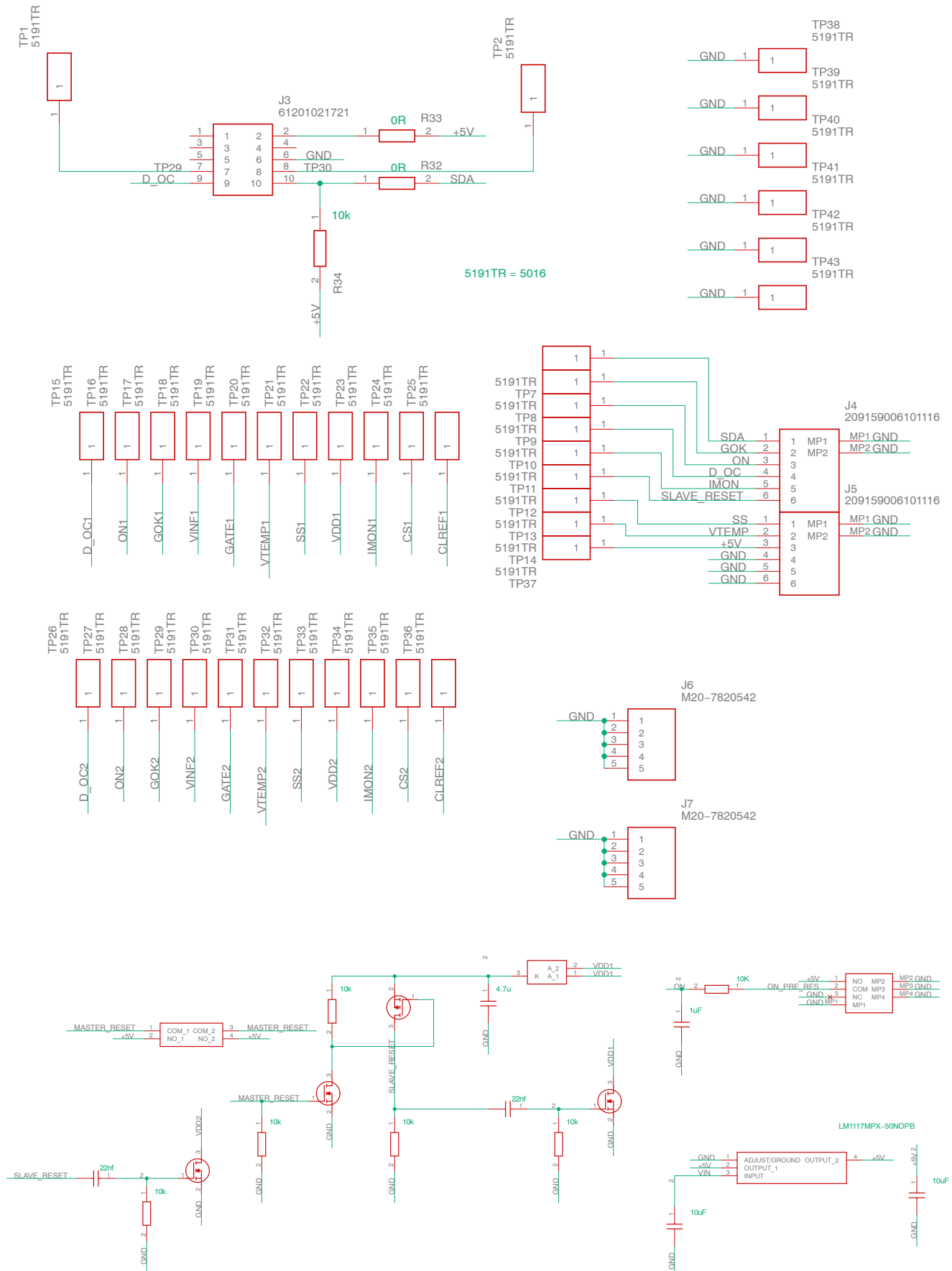
Figure 3. NCP81295GEVB Evaluation Board Schematic, Part 2
