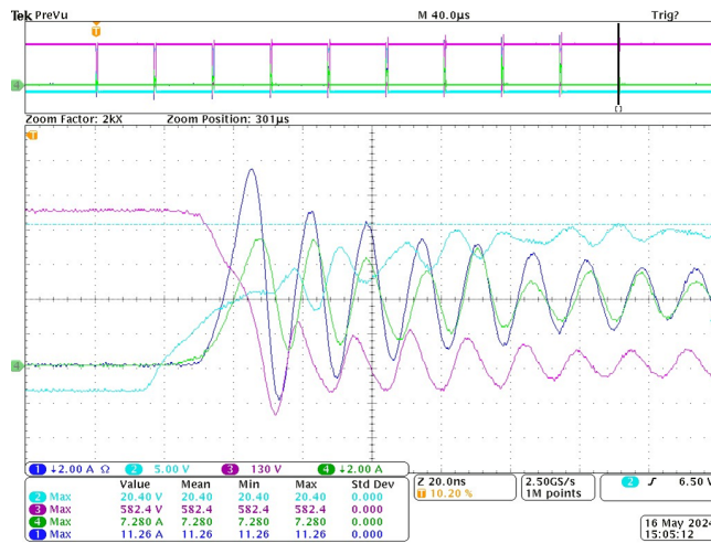
Figure 25. POWER88 – NTMT045N065SC1
