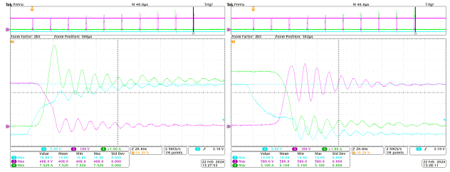
Figure 24. TOLL – NTBL045N065SC1
