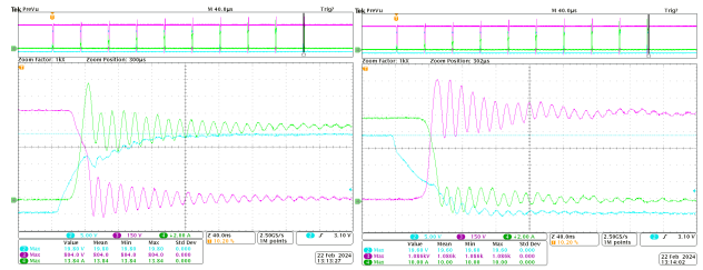
Figure 22. TO247-4L – NTH4L022N120M3S
