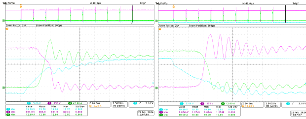
Figure 23. D2PAK-7L – NTBGO22N120M3S
