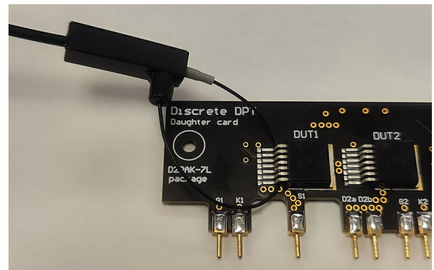
Figure 11. Application Rogowski Current Probe
