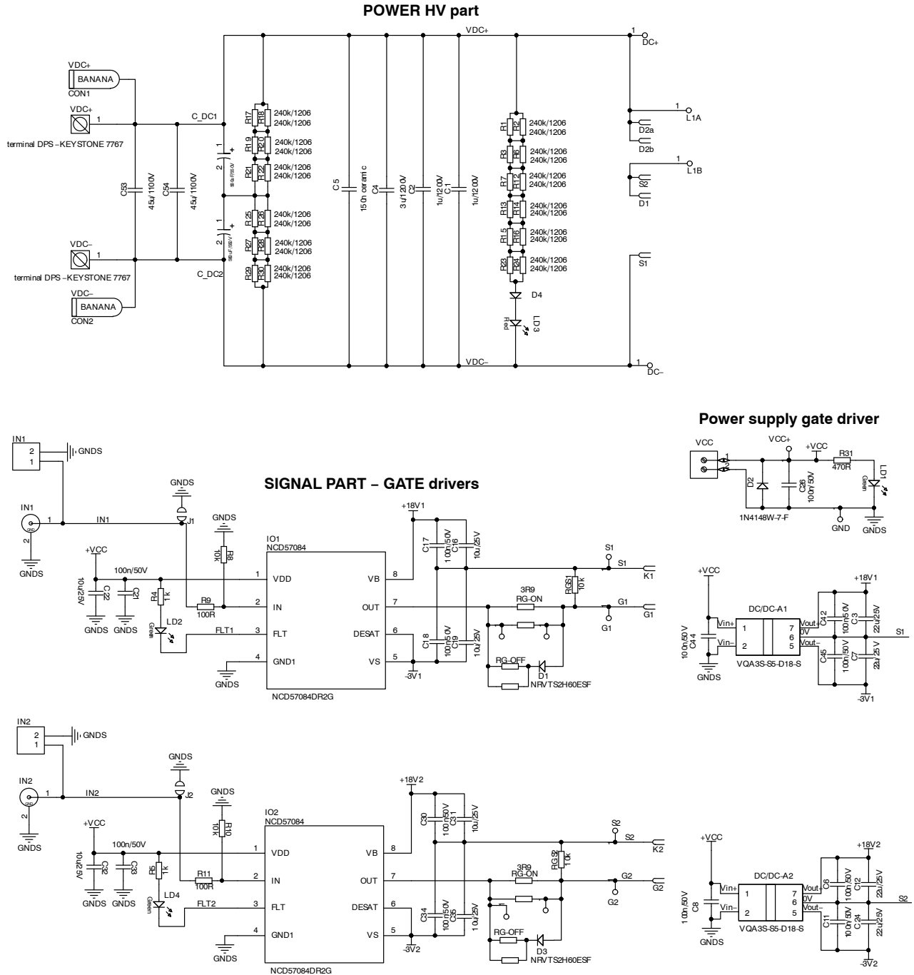
Figure 27. Schematic
