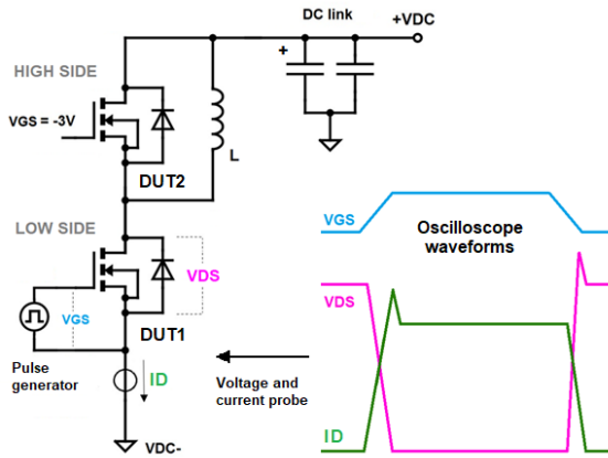
Figure 19. DPT Operation
