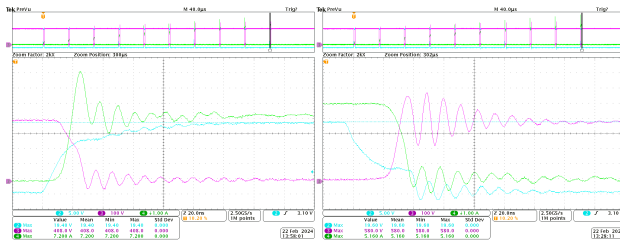
Figure 25. POWER88 – NTMT045N065SC1
