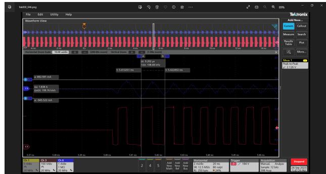
Figure 20. Skip Mode @ 50 V/0.06 A Load
