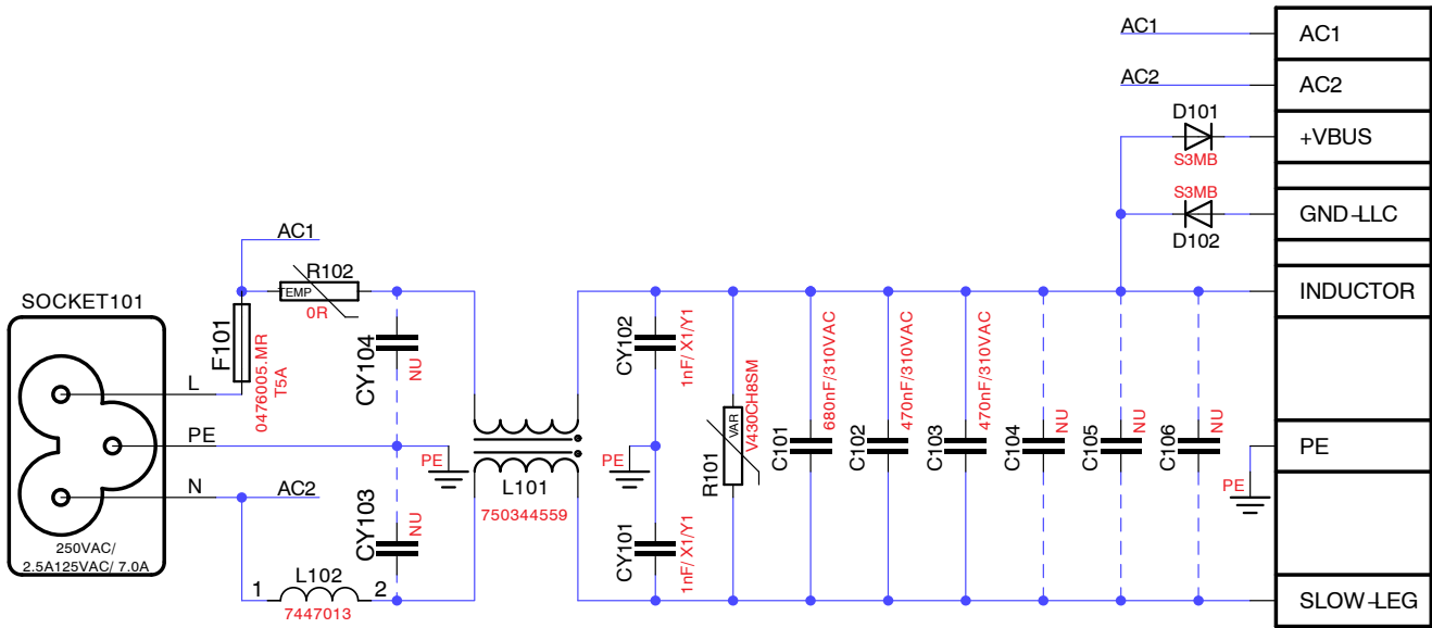
Figure 3. Input EMI Filter Module Schematic Diagram
