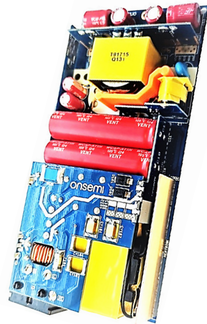
Board Photo
