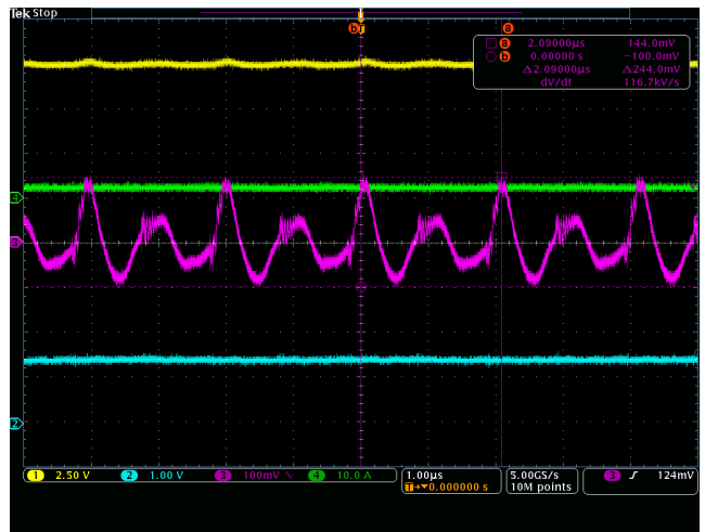
LLC Waveform V_{out} ripple at 2.5 A – detail
