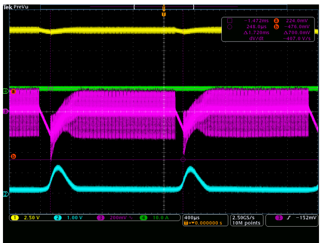
LLC Waveform V_{out} ripple at No-load – bursts detail
