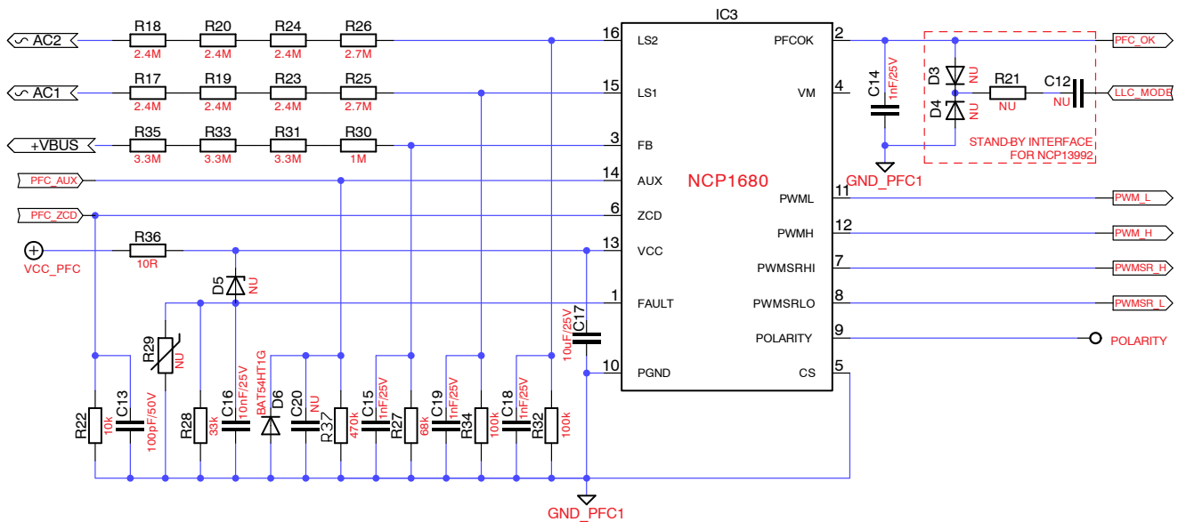
Figure 4. NCP1680 TP PFC Controller Schematic Diagram
