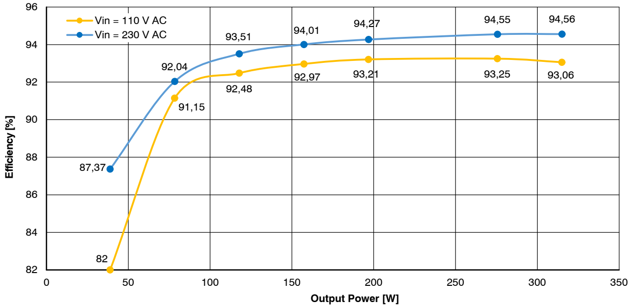
Figure 13. Demo-board Efficiency vs. Load
