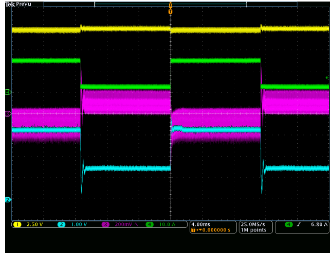
LLC Waveform – Step response 2 A → 15 A
