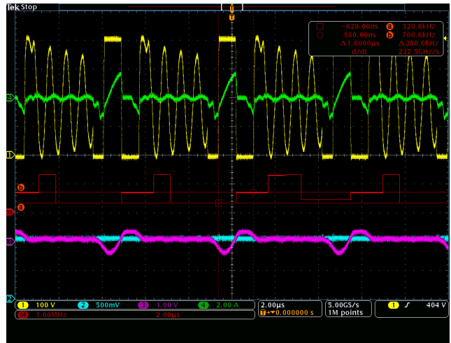
LLC Waveform at Light-load Mode 2 A Load – Package detail
