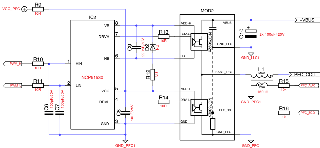
Figure 6. Fast-leg Module with NCP51530 Used as Level Shifter
