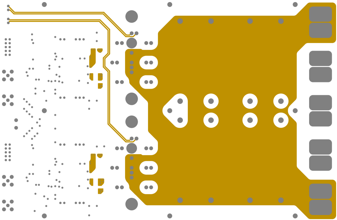
Figure 22. MIDDLE 1 Layer
