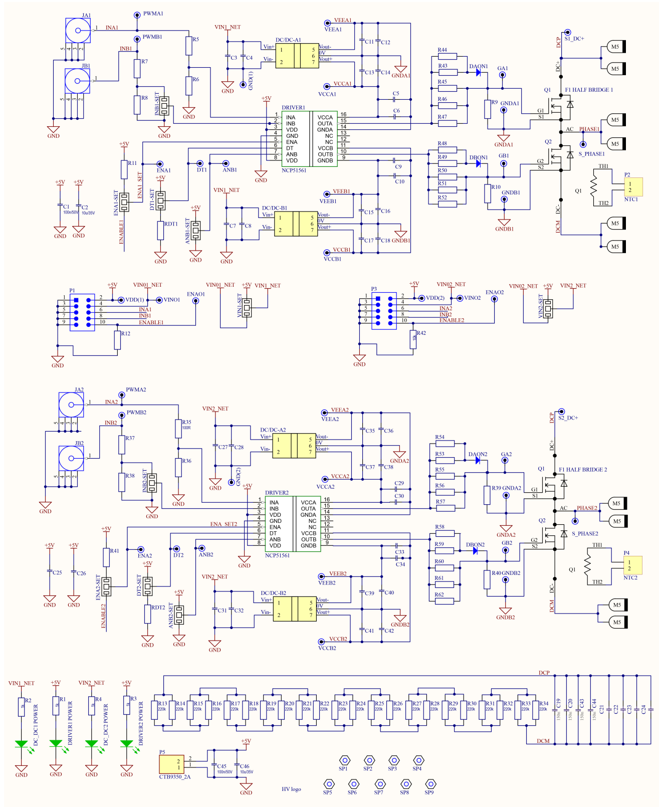
Figure 19. Complete Schematics
