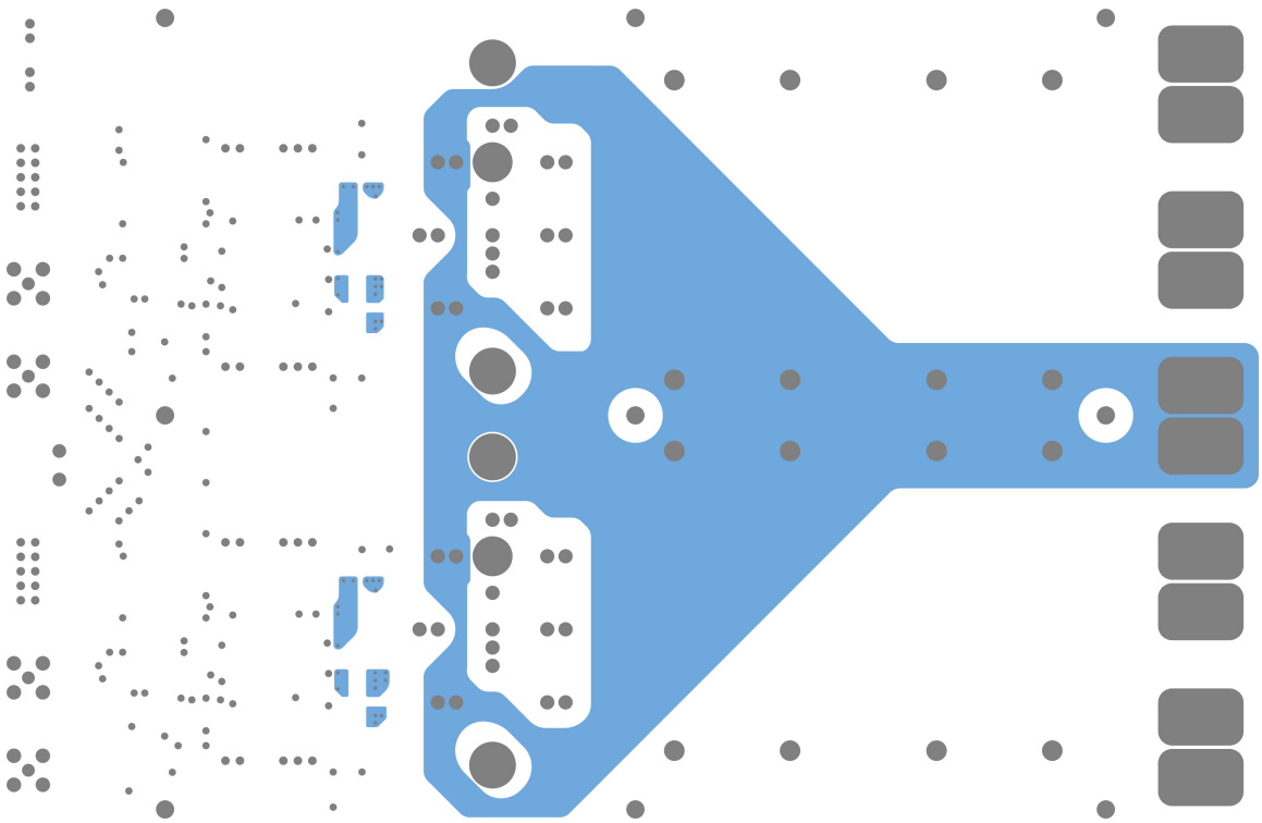
Figure 23. MIDDLE 2 Layer
