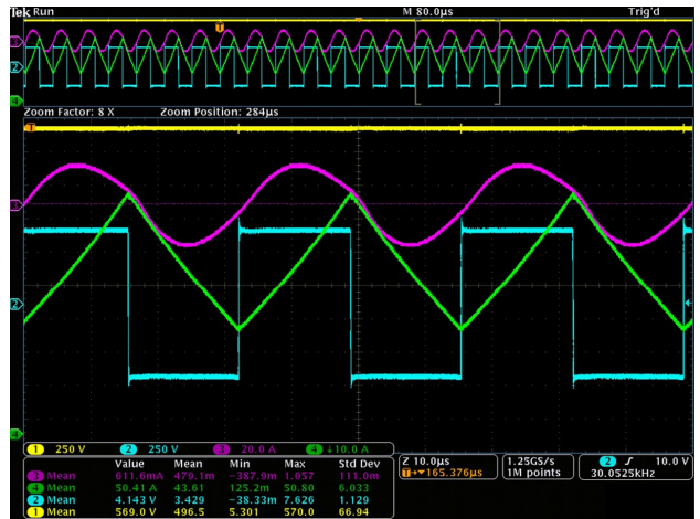
Figure 17. Oscilloscope Waveforms (Yellow V_{DC} link, Red I_C current source, Green I_{Load} , blue V_{Load} )
