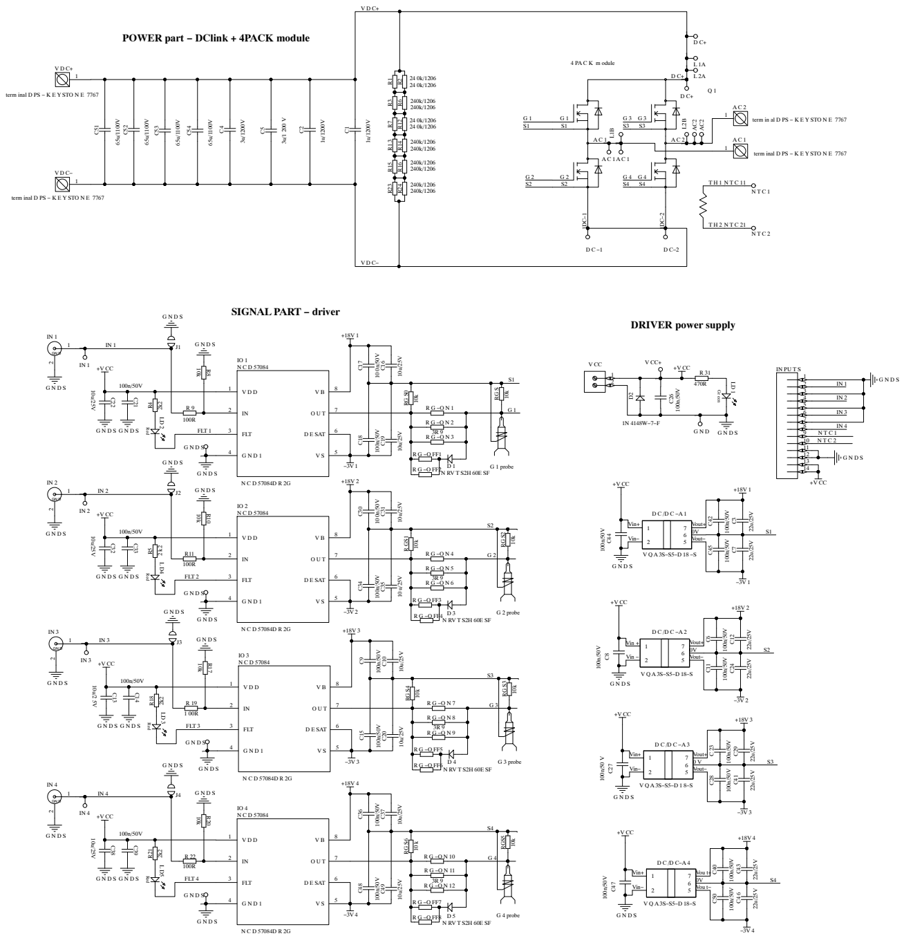
Figure 19. Complete Schematics
