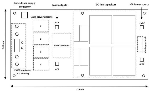
Figure 2. Simplify PCB Block Diagram
