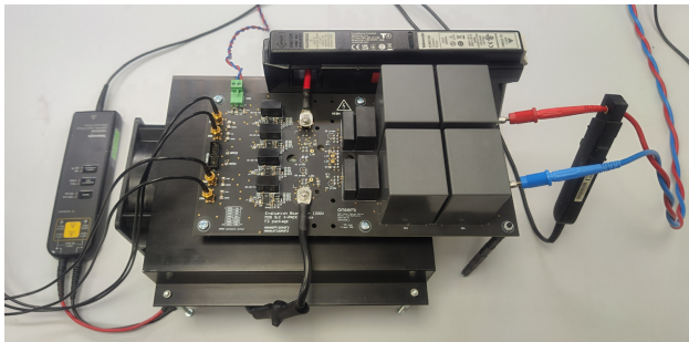
Figure 16. Load Test SETUP
