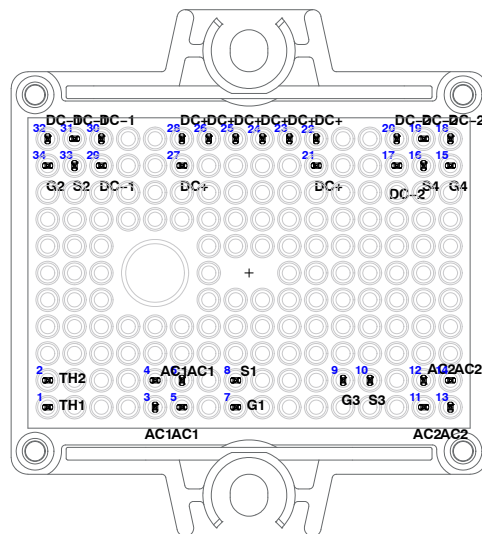
Figure 7. 4PACK Module Schematic and Pinout
