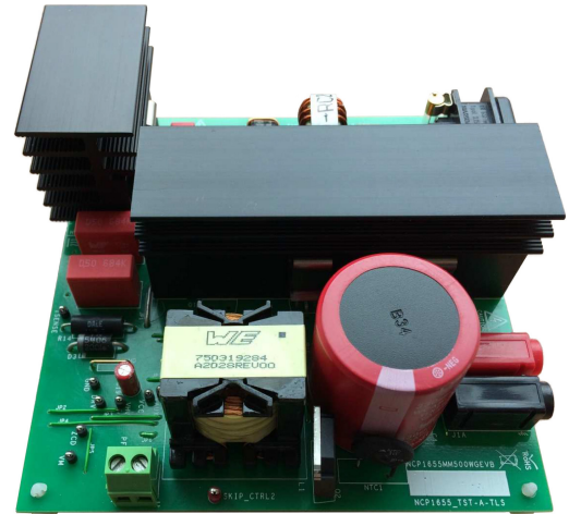
Figure 1. The Wide-mains, 500-W PFC Stage
