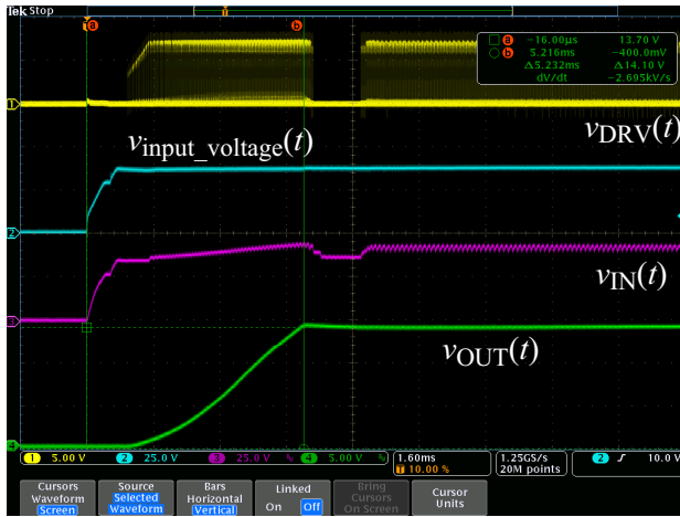
Figure 5. Self-supplied, V_{IN} = 38\text{ V} , I_{OUT} = 0\text{ A} , t_{\text{startup}} = 5.2\text{ ms}
