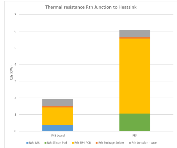
Figure 13. Calculated R_{thJ-H} for FR4 Board and IMS Board
