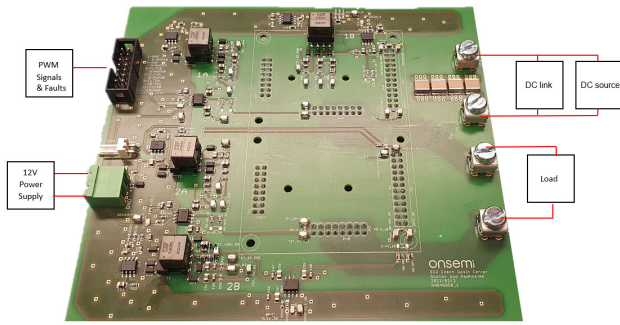
Figure 10. Board Connection
