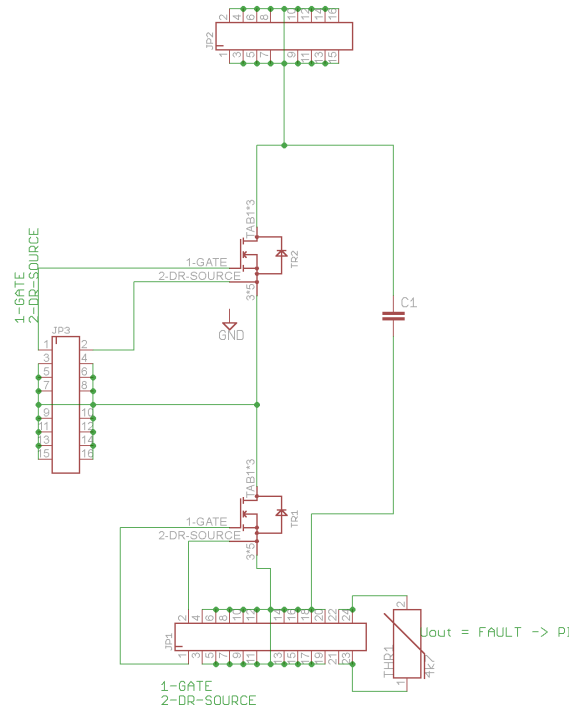
Figure 24. Power Board Schematics
