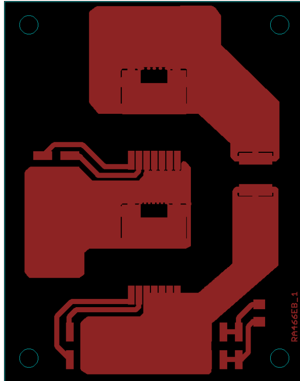
Figure 31. Top Layer
