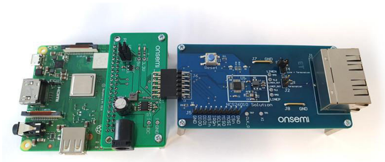
Figure 5. Raspberry Pi 3A+ Connected to the Evaluation Kit. A Kit Consists of an NCN26010BMNEVB and an NCN26010XMNEVB (Revision 1 Boards shown)
