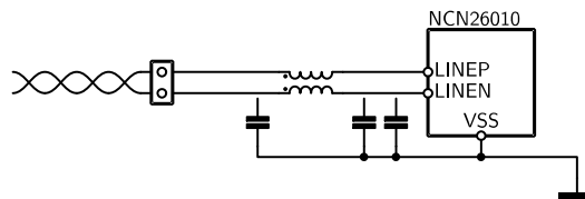
Figure 19. The Ground Plane should be Omitted Until the Common-mode Choke (left) to Avoid Capacitive Coupling (right)
