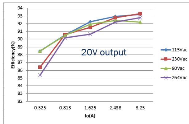
Figure 15. PD_20V Output
