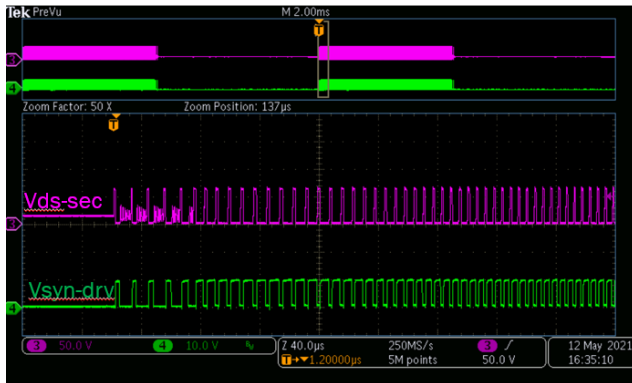
Figure 29. 264 Vac & 15 V, 0 to 3 A (CH3: Vds-sec, CH4: Vsyn-driv)
