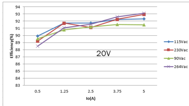
Figure 17. PD_20V Output
