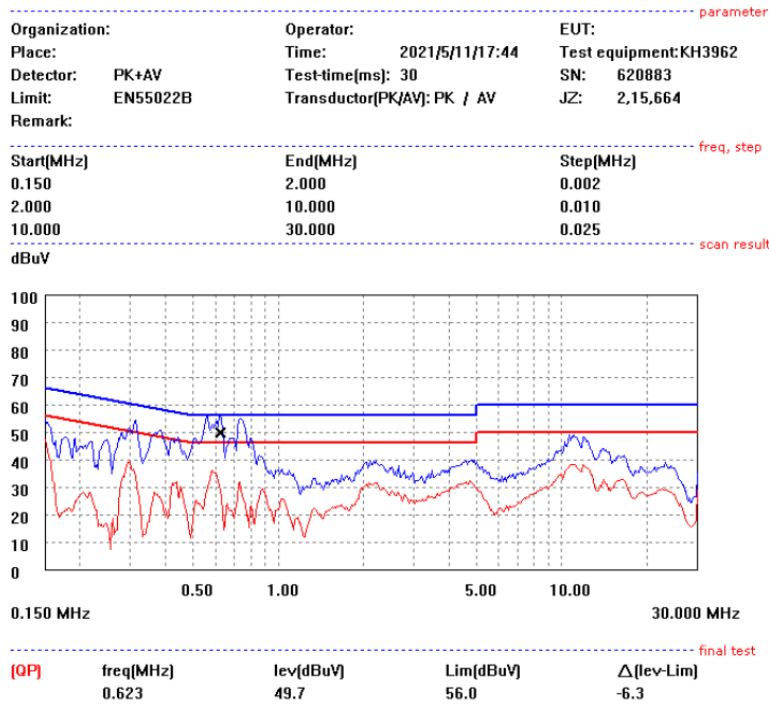
Figure 53. Neutral
