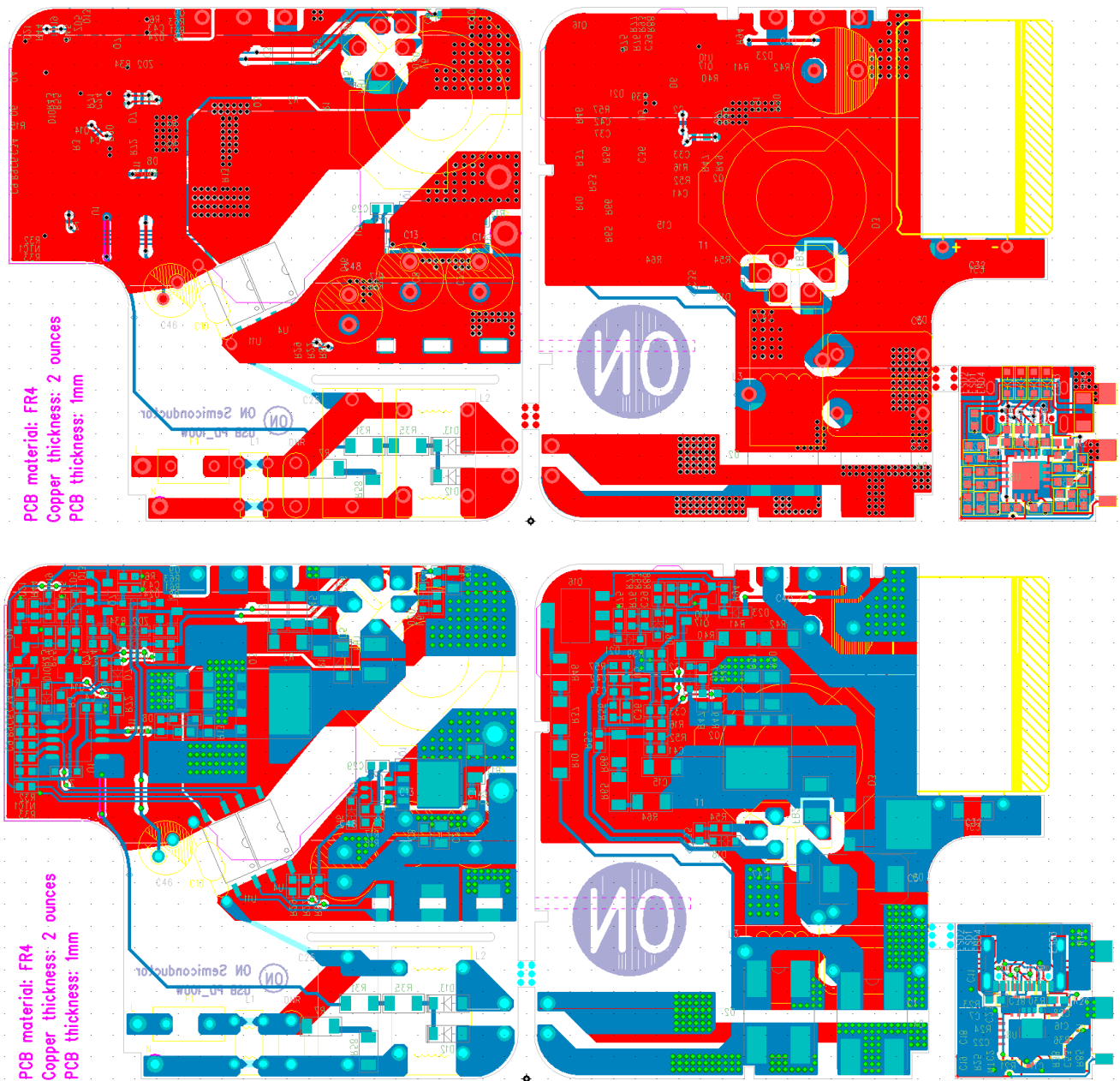
Figure 6. (Top), Top View of PCB
