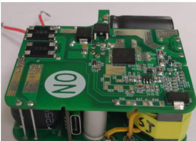
Figure 2. PFC Side View 1 of Demoboard
