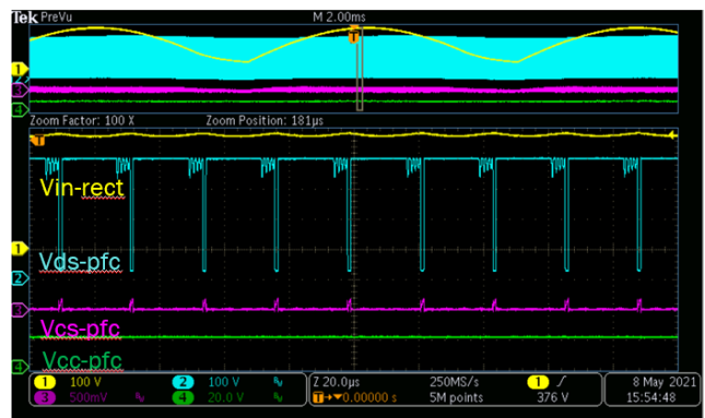
Figure 23. 264 Vac & 20 V 5 A (CH1: Vin-rect, CH2: Vds-pfc, CH3: Vcs-pfc, CH4: Vcc-pfc)
