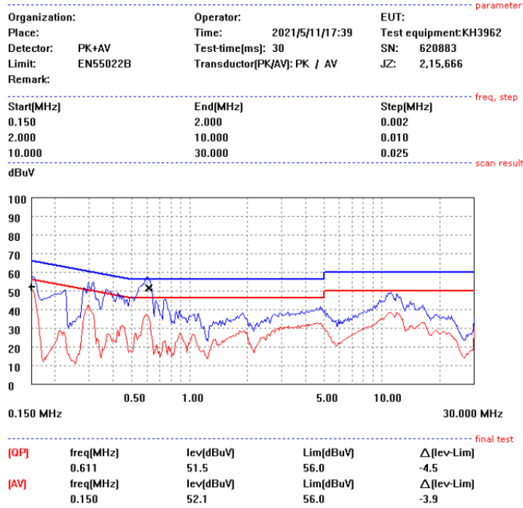
Figure 52. Line
