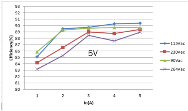
Figure 13. PD_5V Output
