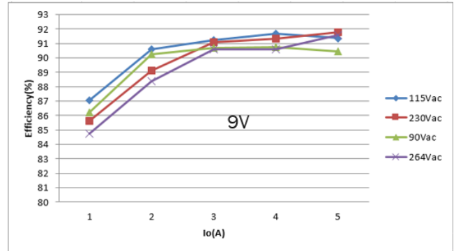
Figure 14. PD_9V Output
