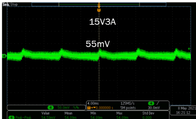
Figure 33. 15 V 3 A Output (CH4: Vo)
