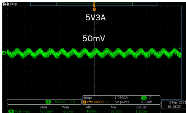
Figure 31. 5 V 3 A Output (CH4: Vo)
