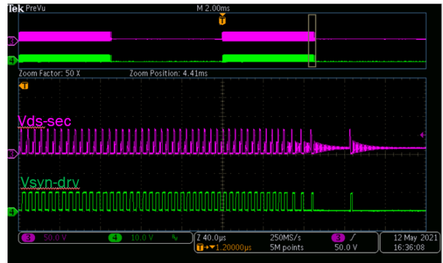
Figure 30. 264 Vac & 15 V, 3 A to 0 (CH3: Vds-sec, CH4: Vsyn-driv)
