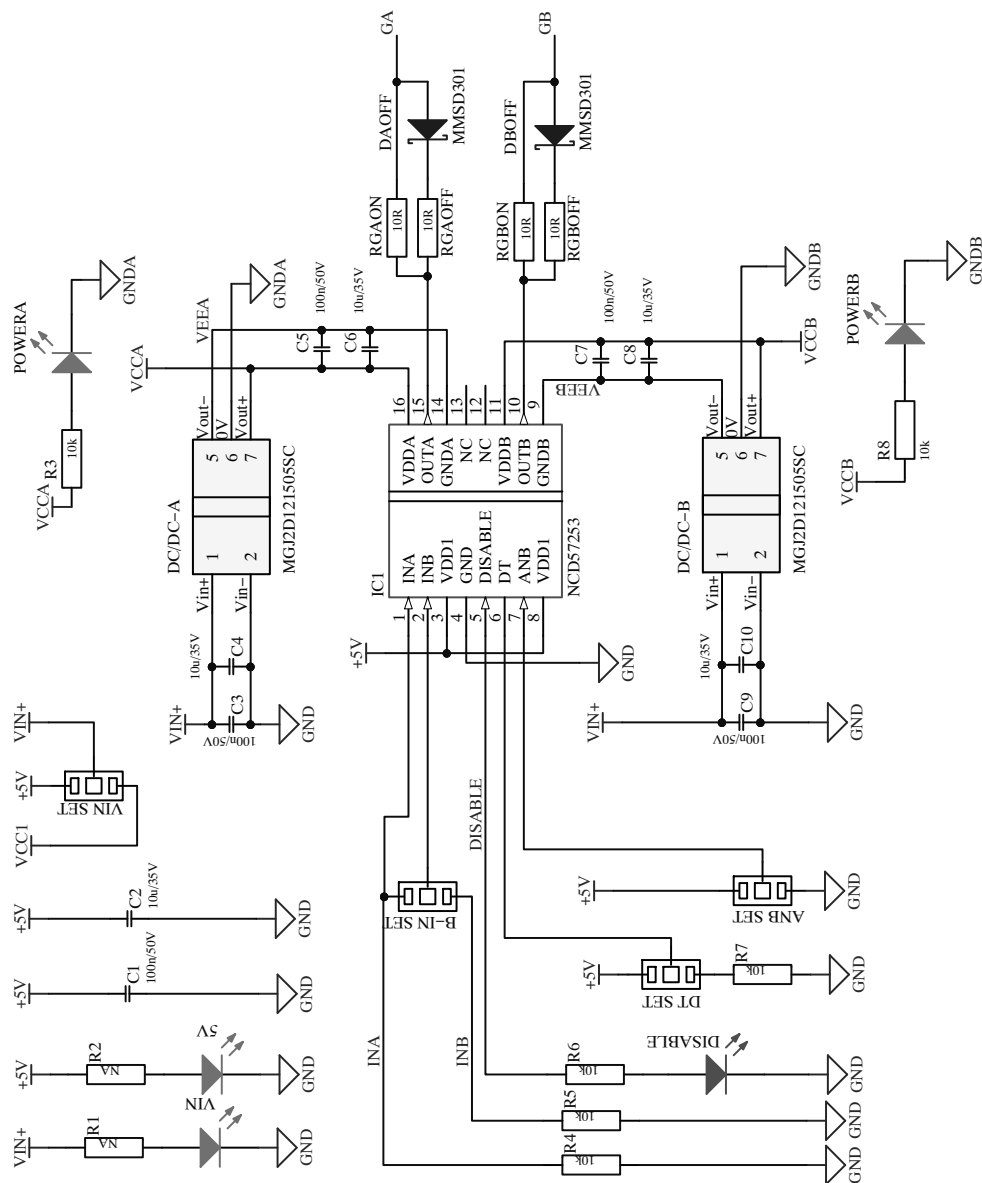
Figure 14. Schematic
