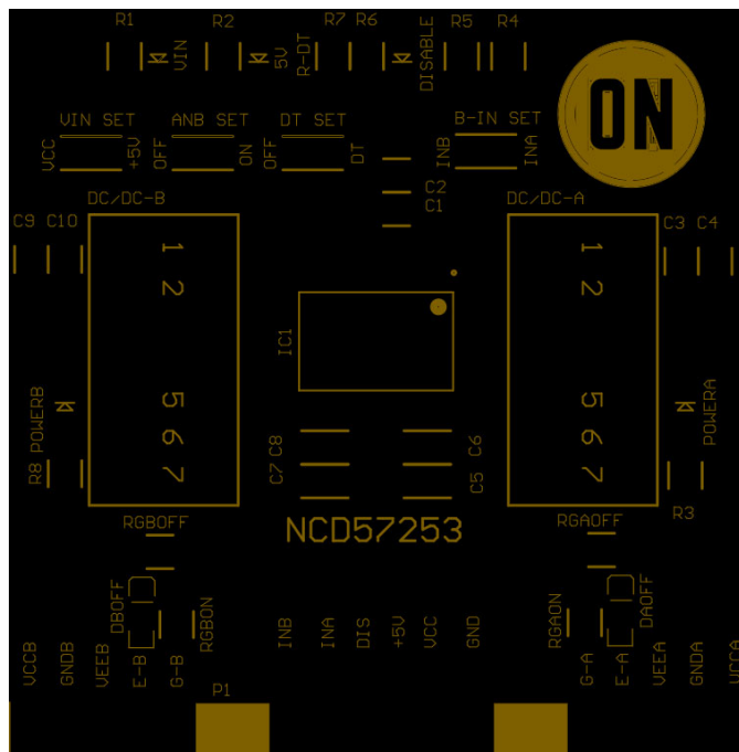
Figure 16. TOP Overlay
