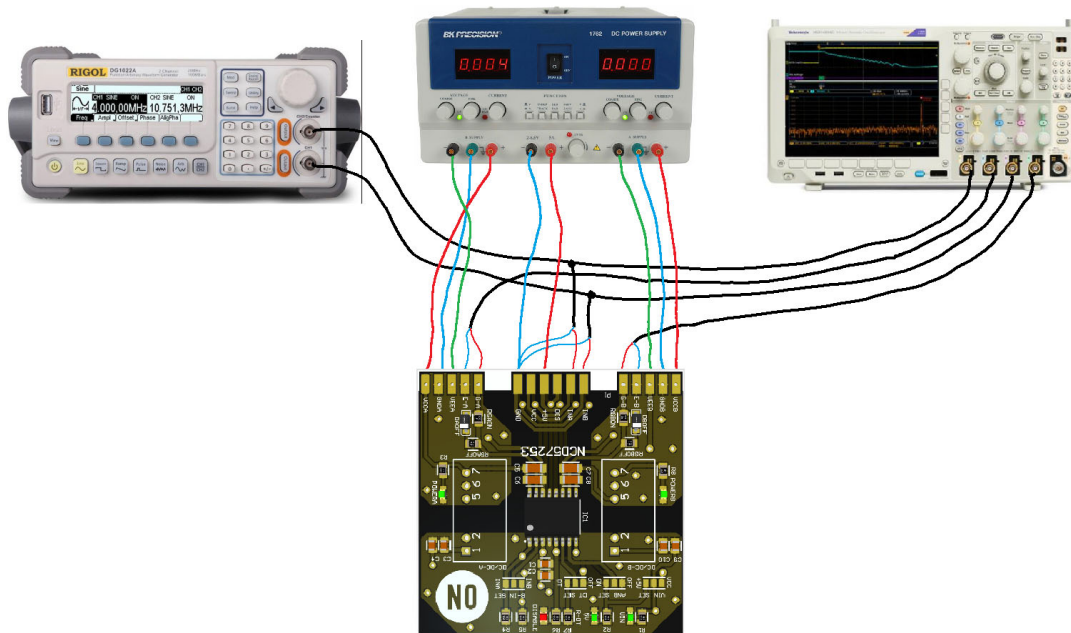
Figure 4. External Power Supply (No On Board DC-DC Converters)
