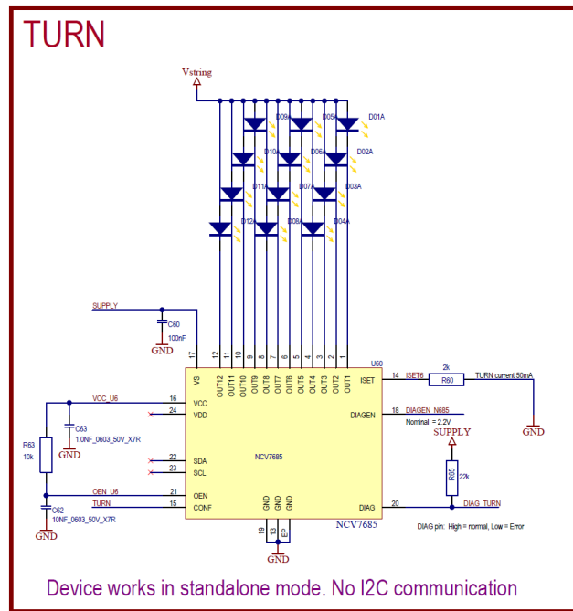
Figure 12. Schematic of the NCV7685LOWR1GEVB Variant Part A
