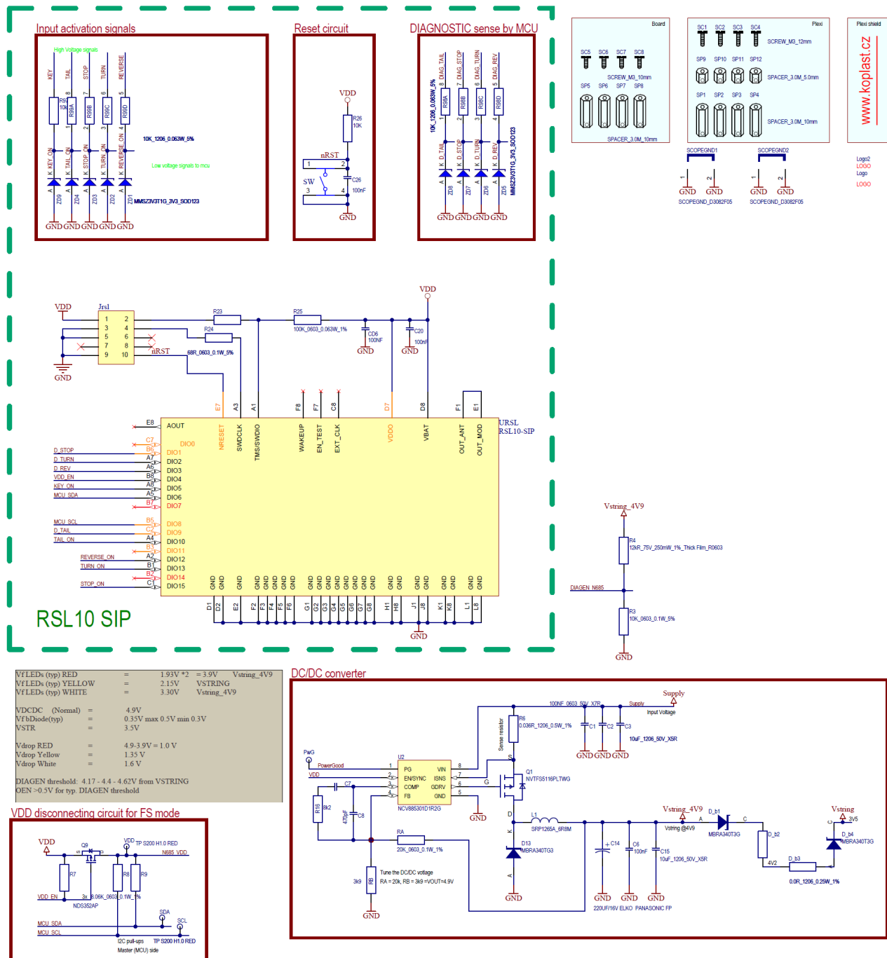
Figure 15. Schematic of the NCV7685MIDR1GEVB Part B
