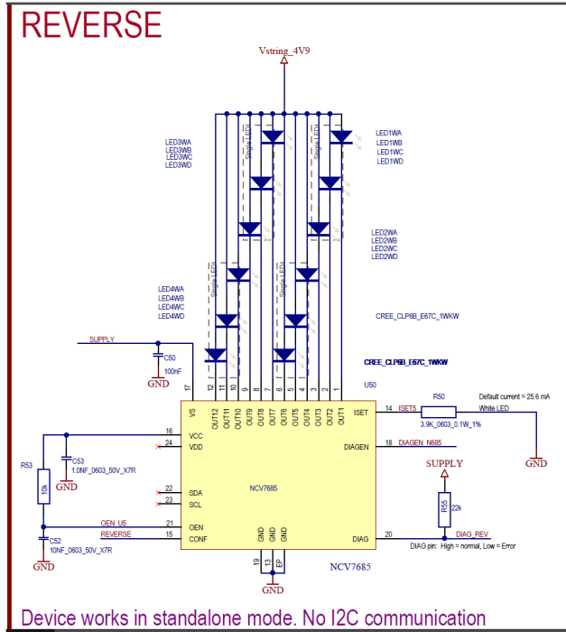
Figure 12. Schematic of the NCV7685LOWR1GEVB Variant Part A
