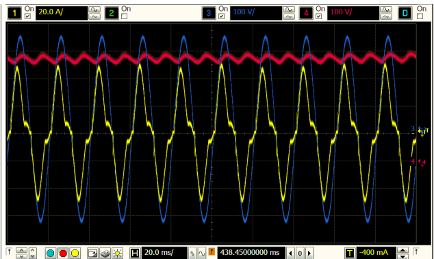
Figure 25. Vin 220 V, Pin = 6.6 kW
