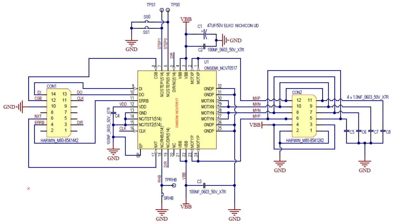
Figure 7. Schematic of NCV70517/NCV70514 Daughter Board
