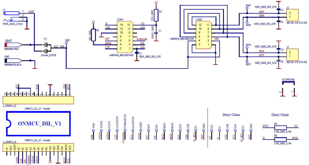
Figure 6. Schematic of SPI Stepper Driver EVK Mother Board
