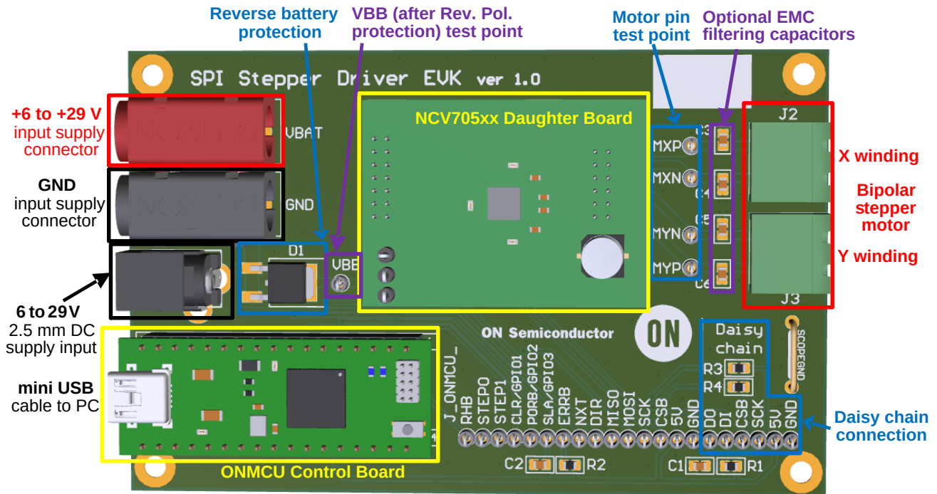
Figure 2. NCV705XXGEVK Micro-stepping Motor Driver Evaluation Board Picture
