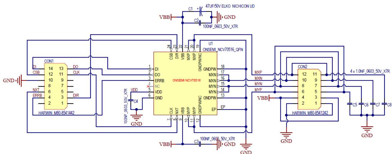
Figure 8. Schematic of NCV70516 Daughter Board
