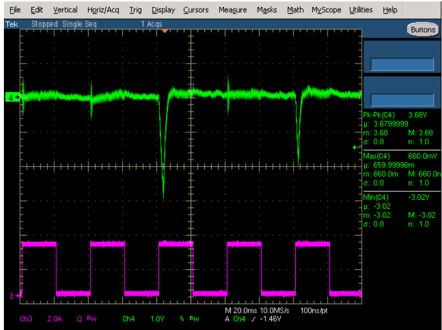
Figure 45. 48 Vin 15 Vout Transient Response
