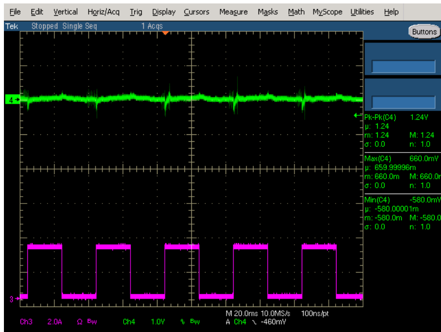
Figure 36. 48 Vin 5 Vout Transient Response
