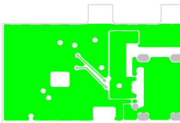
Figure 10. Daughter Card Inner Layer 2
