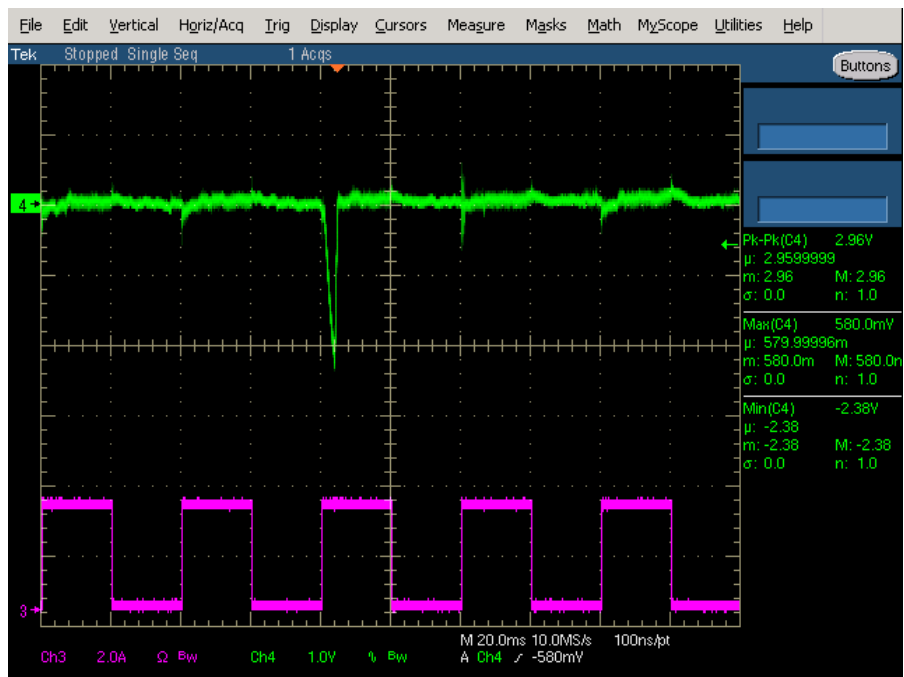
Figure 42. 48 Vin 12 Vout Transient Response
