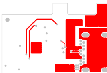
Figure 11. Daughter Card Bottom Layer
