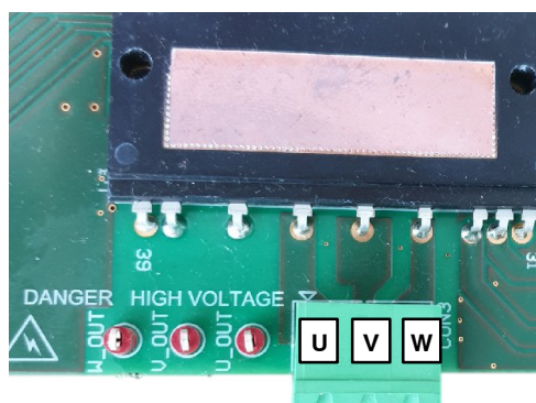
Figure 17. Inverter Output Voltage Phase Connector
