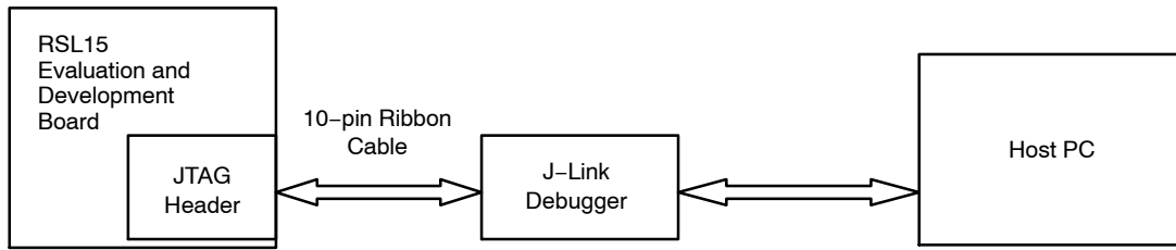
Figure 3. J-Link Connection
