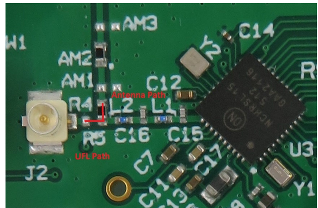
Figure 4. Selection of RF Path Through R4, R5 (0 \Omega Resistors)
