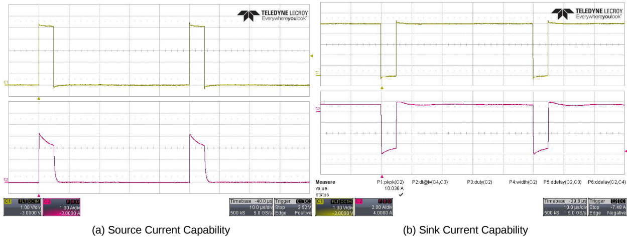
(a) Source Current Capability
