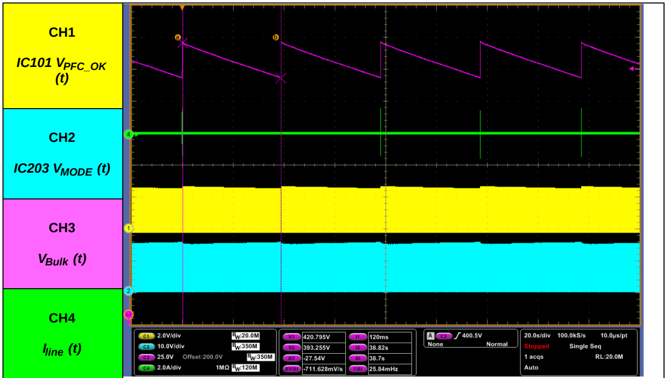
Figure 48. 110 V AC/ No-load, PFC Soft-skip mode – V_{Bulk} Hiccups
