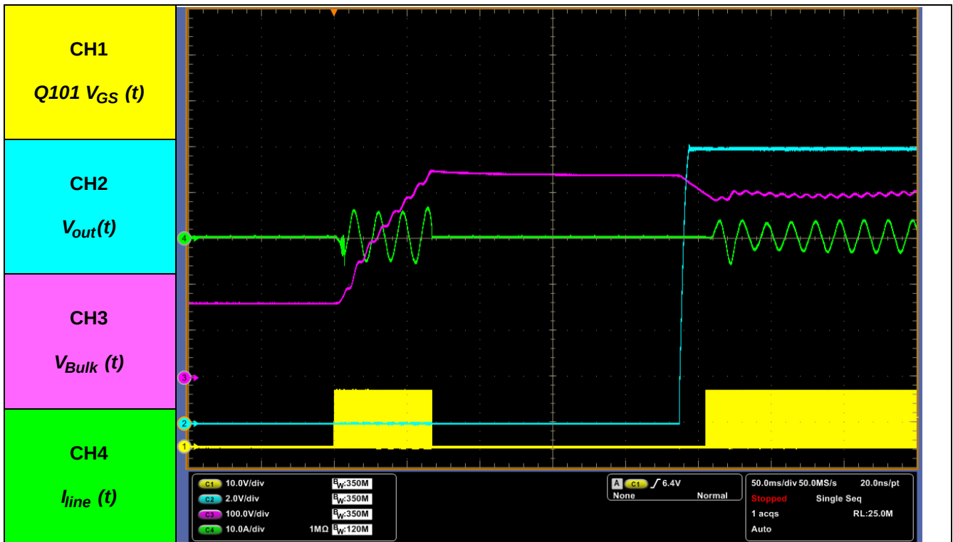
Figure 37. 110 V AC/ Load 20 A, PFC/ LLC START-UP (No inrush limiter)
