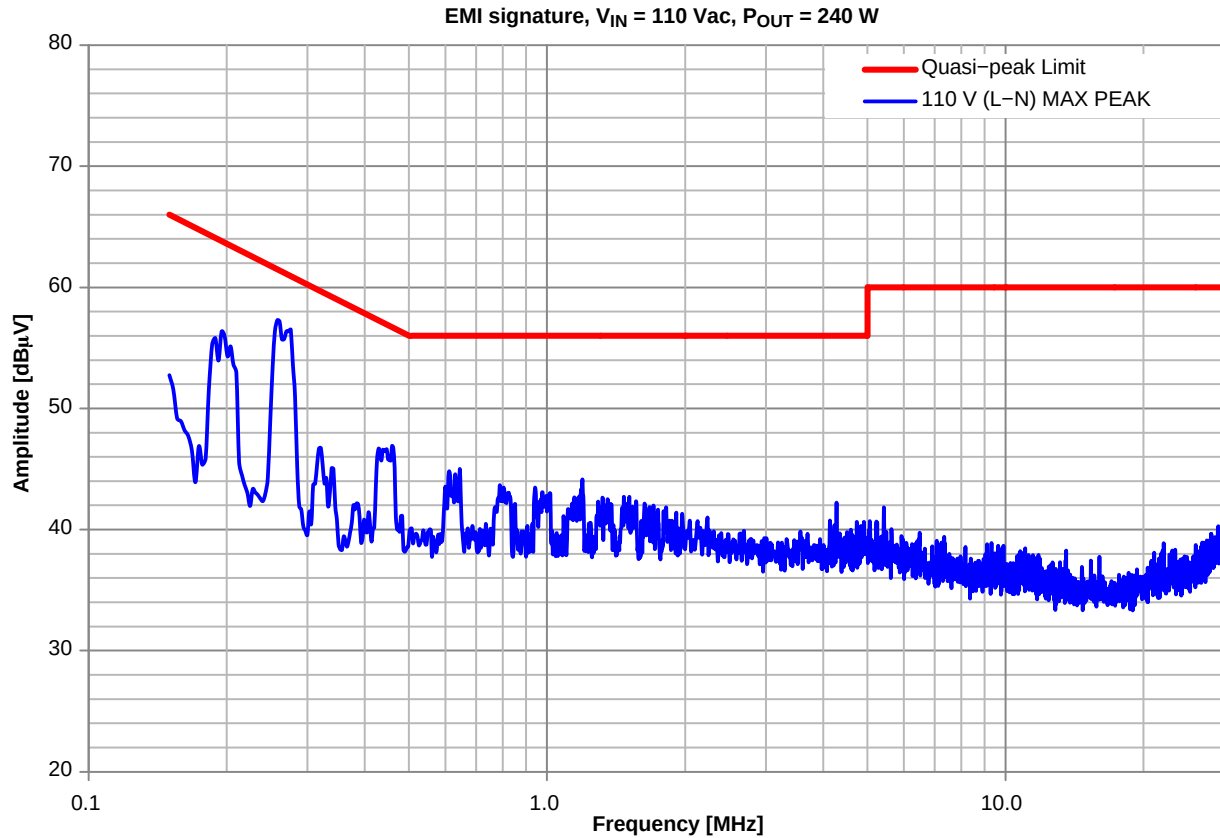
Figure 16. EMI Signature Comparison @ 110 VAC & Full-load (measured MAX Peak)
