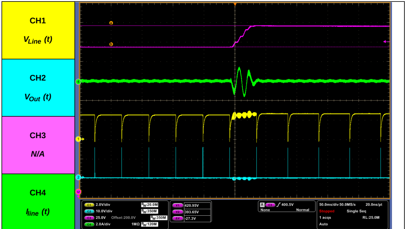
Figure 49. 110 V AC/ No-load, PFC Soft-skip mode – V_{Bulk} Hiccups/ PFC Burst detail
