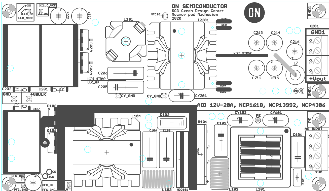
Figure 5. Evaluation Board – Top Side Components
