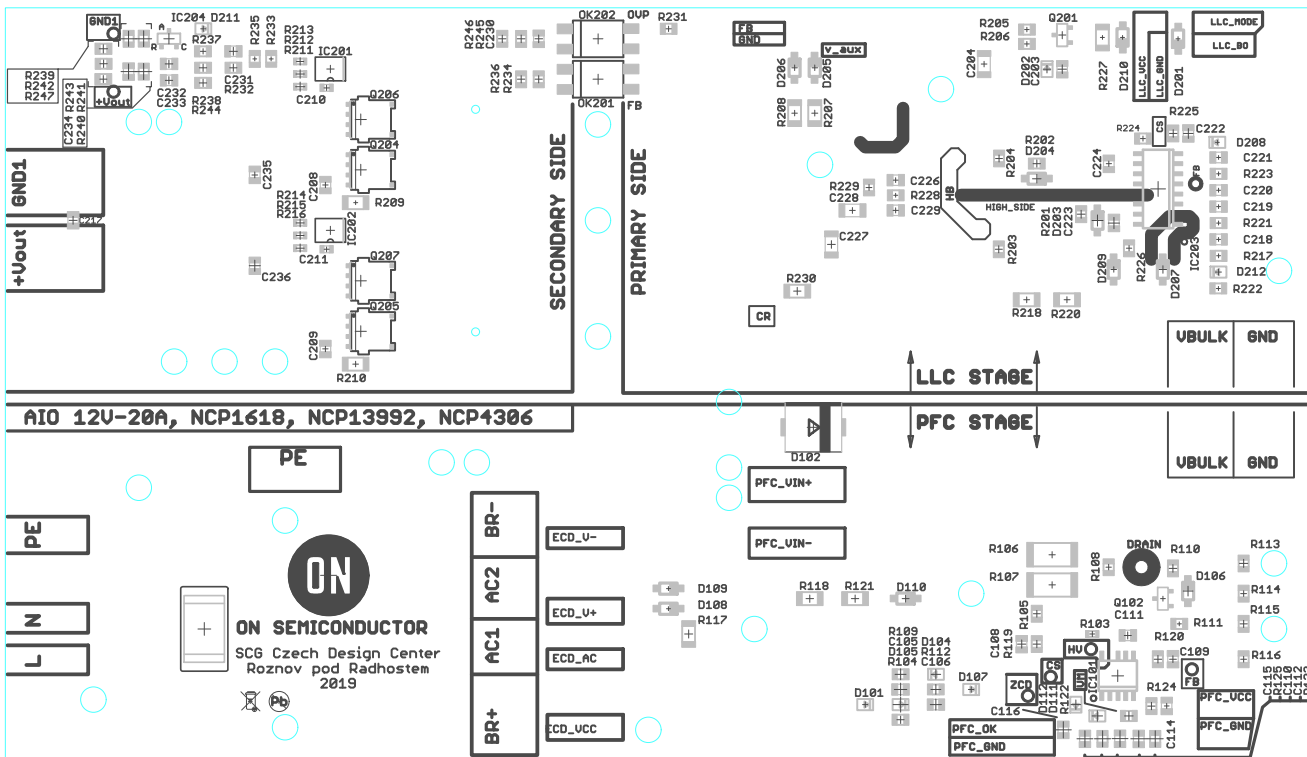
Figure 6. Evaluation Board – Bottom Side Components
