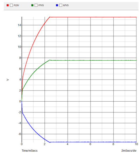
Figure 17. Output Voltages for Vin = 15 V
