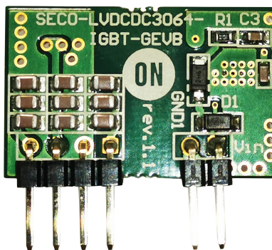
Figure 1. Board Layout
