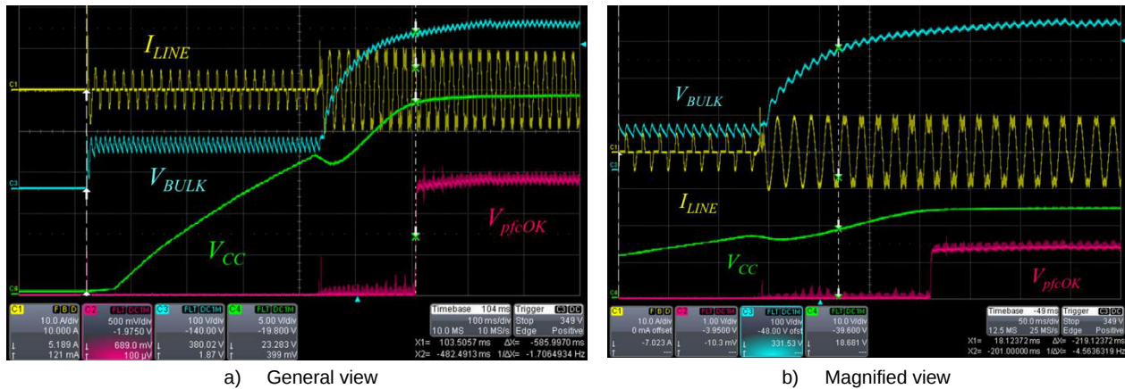
Figure 10. Startup Sequence at Full Load, Low Line
