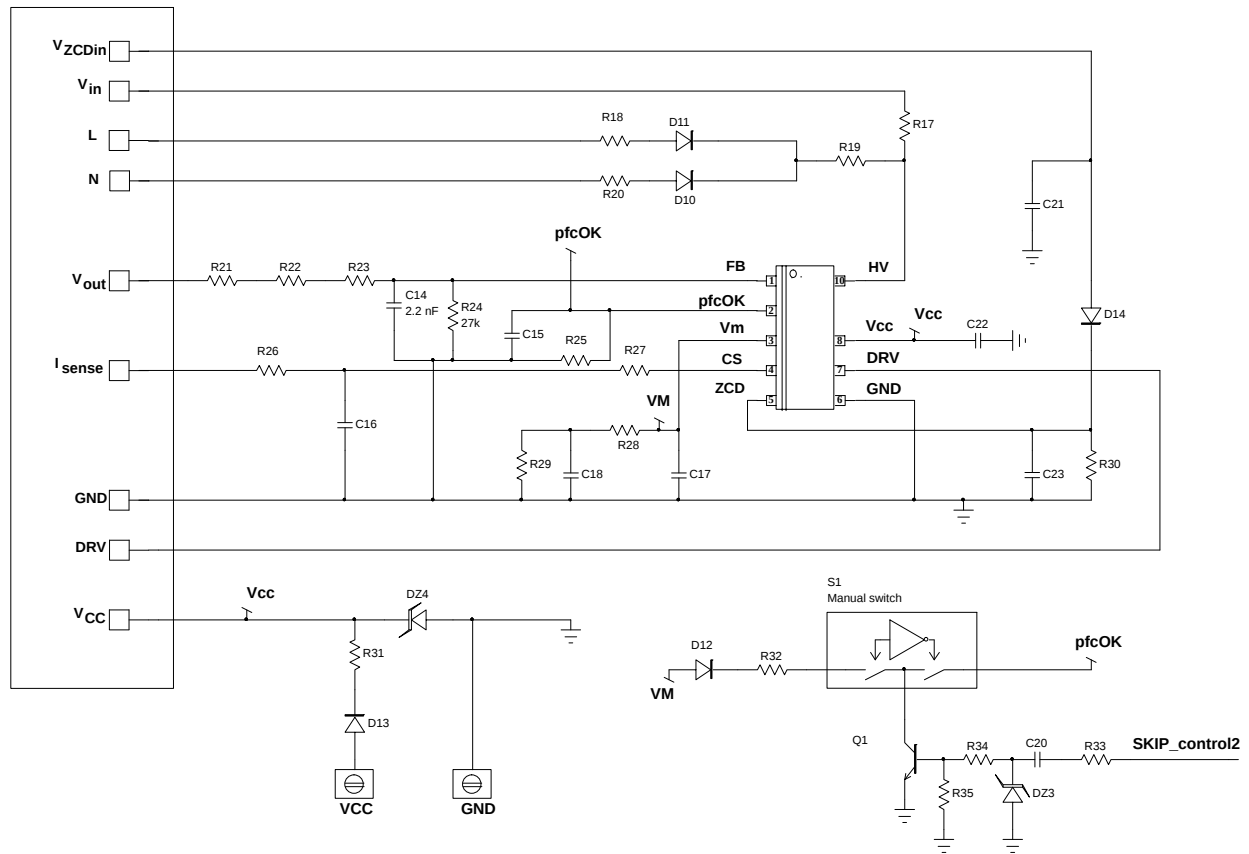
Figure 21. Control Section and Circuitry for Soft-SKIP Testing
