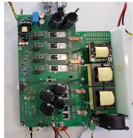
Figure 2. LLC Board Photo
