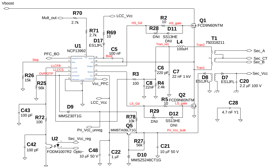
Figure 5. Power Stage
