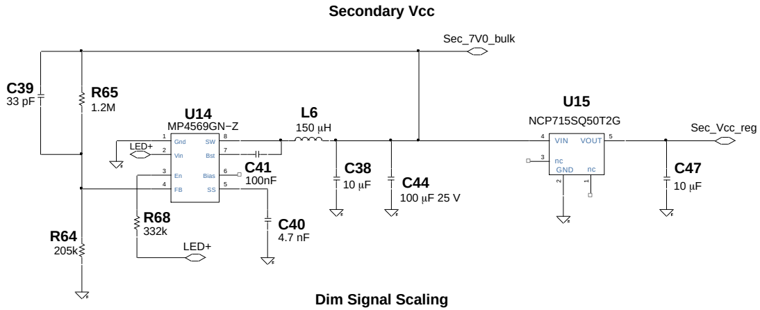
Figure 8. Secondary Dim Interface Circuit
