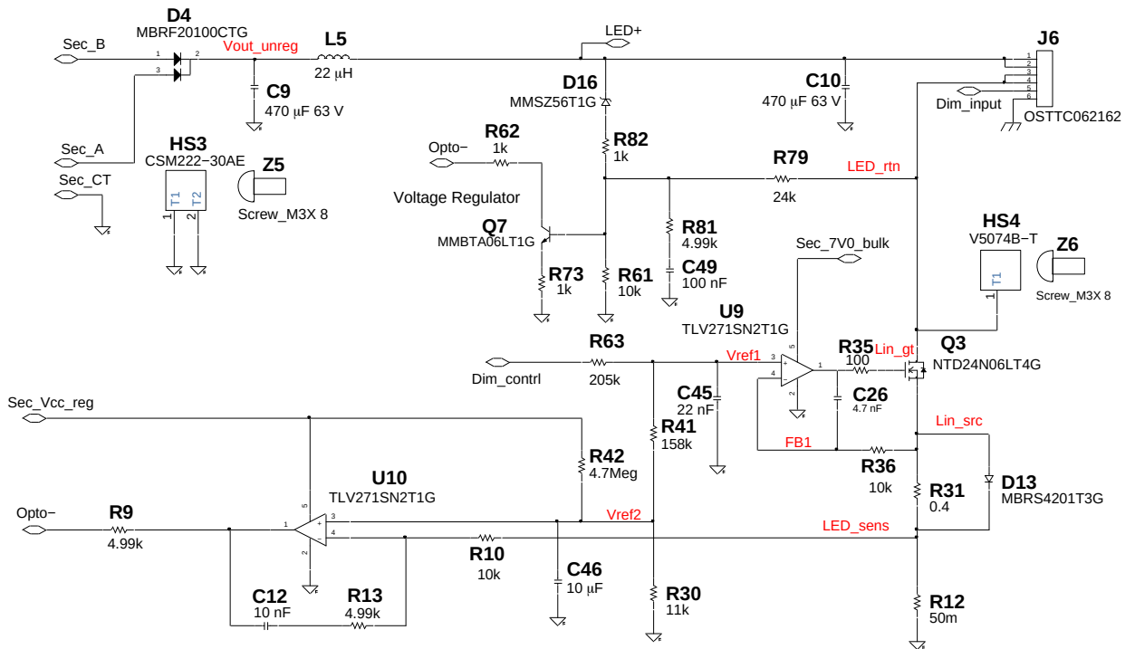
Figure 6. Output Circuit
