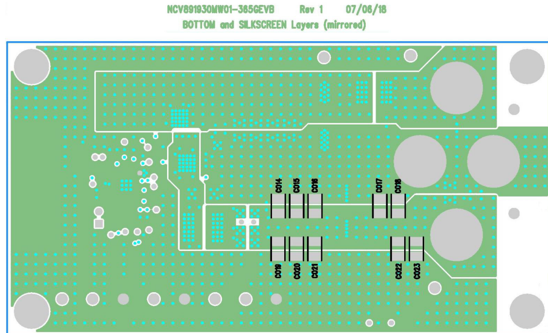
Figure 15. NCV8x1930MW0x-xxxGEVB PCB Layout – BOTTOM (NCV891930MW01-365GEVB Shown)
