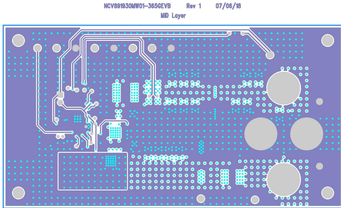
Figure 14. NCV8x1930MW0x-xxxGEVB PCB Layout – MID (NCV891930MW01-365GEVB Shown)
