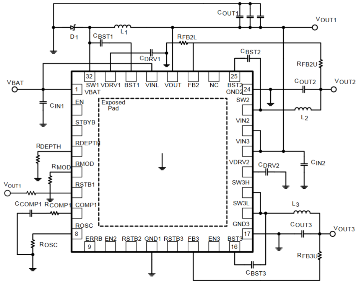
Figure 3. Typical Application
