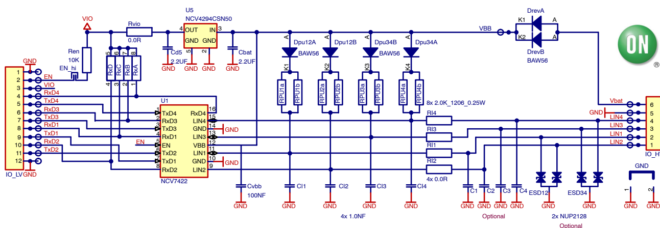
Figure 1. NCV7424 Evaluation Board Schematic
