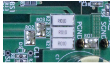
Figure 19. One Shunt Resistance Detection
