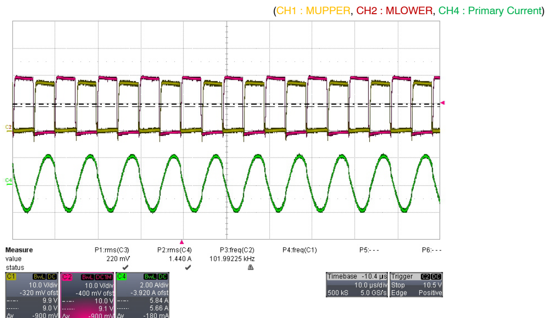
Figure 15. LLC Operation Waveforms
