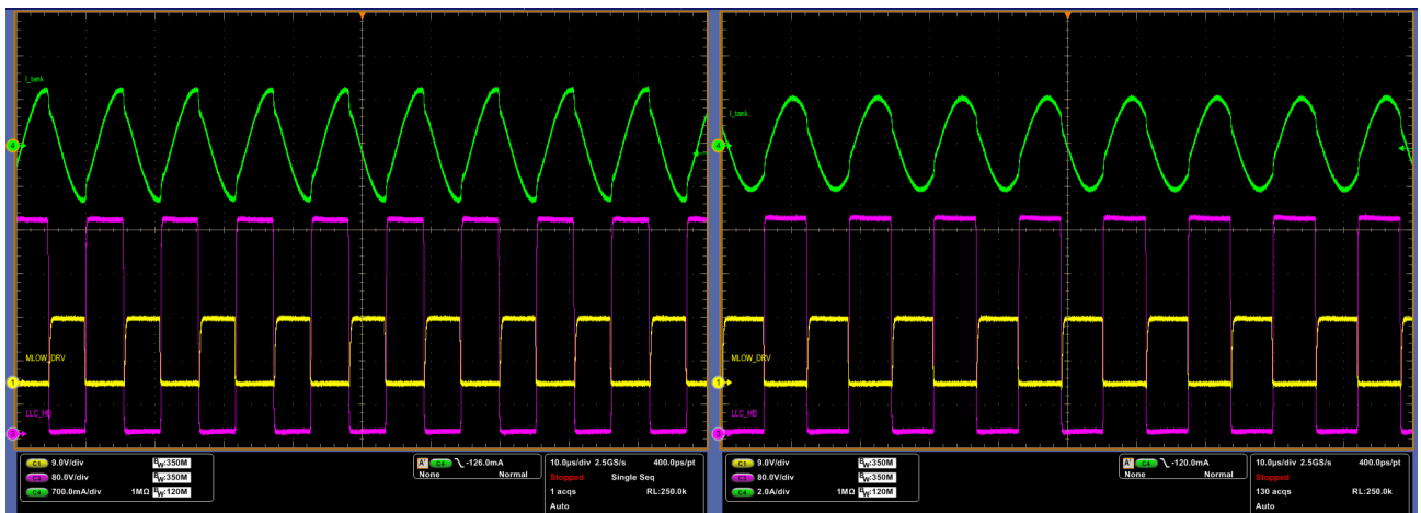
CH1 – LLC Low Side MOSFET Gate-Drive Voltage
