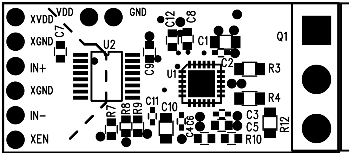
Figure 4. Top Assembly
