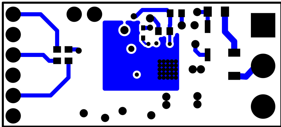
Figure 9. Bottom Layer
