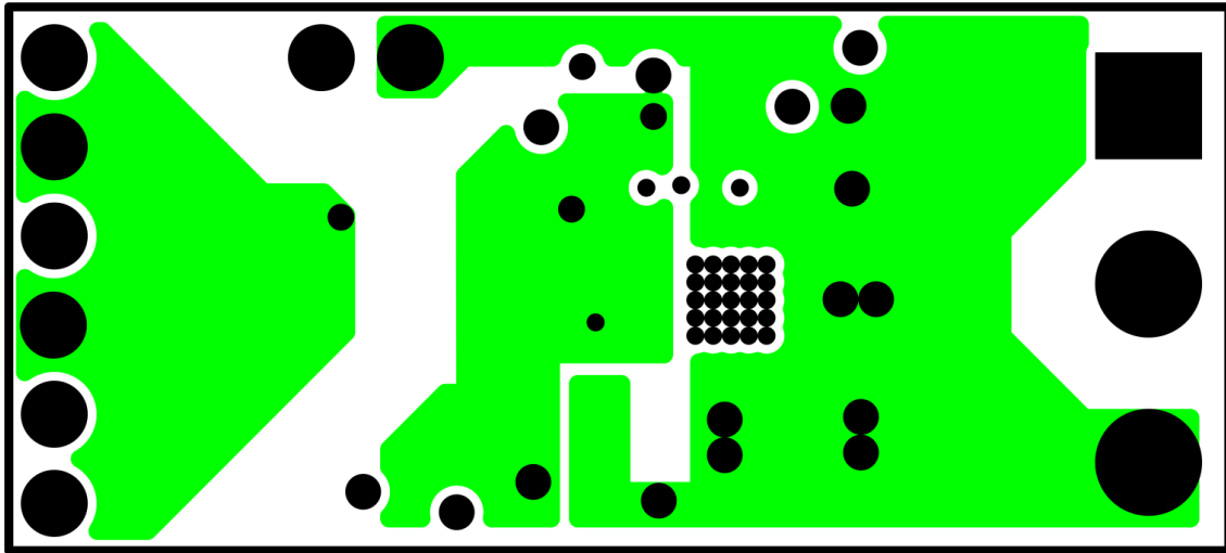
Figure 7. Layer 2
