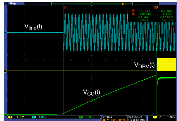
Figure 21. Startup Time – V_{IN} = 120 \text{ V} , t_{startup} = 1.1 \text{ s}
