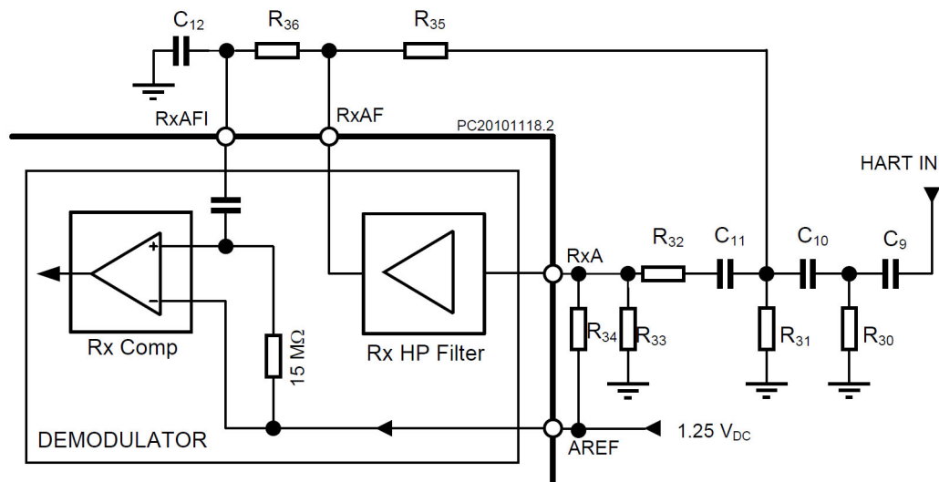
Figure 16. Receive Filter
