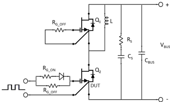
Figure 23. Schematic of the Half-Bridge Mode Switching Test Circuit. Note, a Bus RC Snubber ( R_S = 2.5\text{ }\Omega , C_S = 100\text{ nF} ) is Used to Reduce the Power Loop High Frequency Oscillations.
