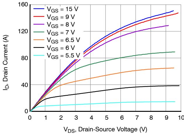
Figure 3. Typical Output Characteristics at T_J = 175^\circ\text{C} , t_p < 250\ \mu\text{s}
