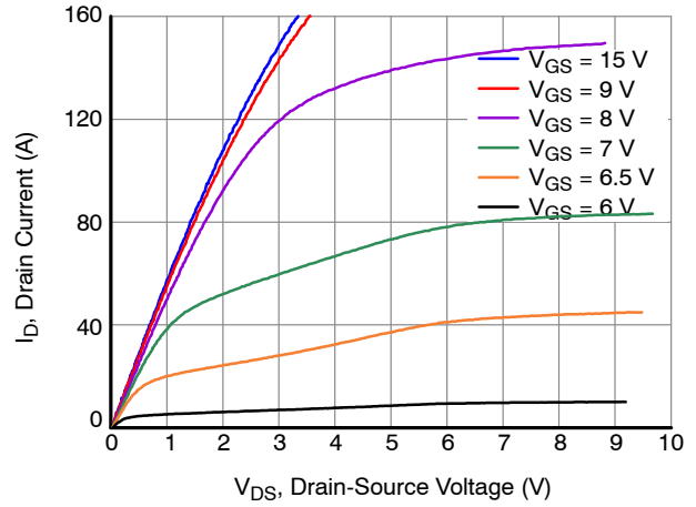
Figure 2. Typical Output Characteristics at T_J = 25^\circ\text{C} , t_p < 250\ \mu\text{s}
