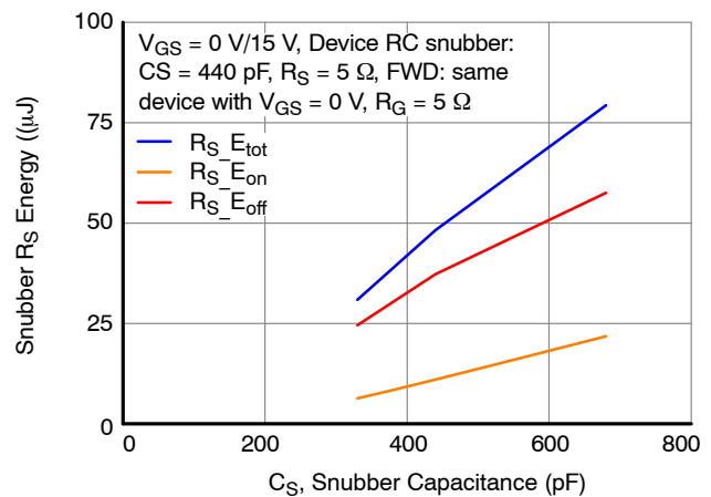
Figure 24. RC Snubber Energy Losses vs. Snubber Capacitance C_S at V_{DS} = 400\text{ V} , I_D = 60\text{ A} and T_J = 25\text{ }^\circ\text{C}
