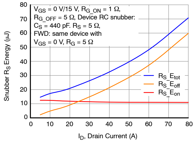
Figure 20. RC Snubber Energy Loss vs. Drain Current at V_{DS} = 400\text{ V} and T_J = 25\text{ }^\circ\text{C}
