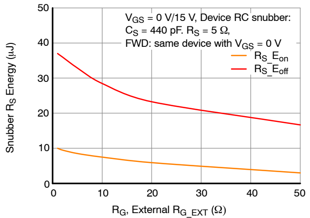
Figure 22. RC Snubber Energy Losses vs. R_{G\_EXT} at V_{DS} = 400\text{ V} , I_D = 60\text{ A} and T_J = 25\text{ }^\circ\text{C}
