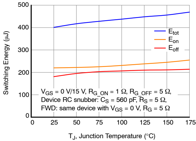
Figure 25. Clamped Inductive Switching Energy vs. Junction Temperature at V_{DS} = 400 \text{ V} and I_D = 70 \text{ A}
