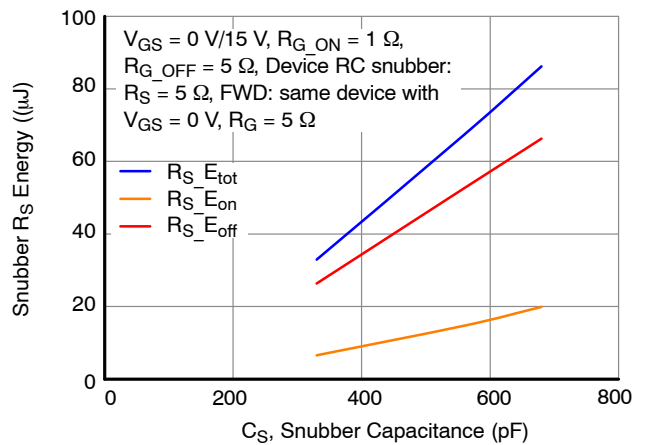
Figure 24. RC Snubber Energy Losses vs. Snubber Capacitance C_S at V_{DS} = 400\text{ V} , I_D = 70\text{ A} and T_J = 25\text{ }^\circ\text{C}
