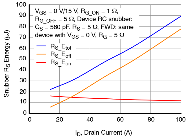
Figure 20. RC Snubber Energy Loss vs. Drain Current at V_{DS} = 400\text{ V} and T_J = 25\text{ }^\circ\text{C}
