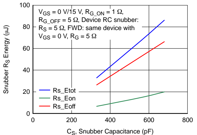
Figure 24. RC Snubber Energy Loss vs. Snubber Capacitance C_S at V_{DS} = 400\text{ V} , I_D = 70\text{ A} , and T_J = 25\text{ }^\circ\text{C}
