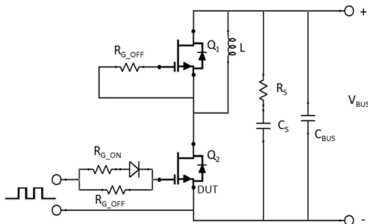
Figure 29. Schematic of the Half-Bridge Mode Switching Test Circuit. Note, a Bus RC Snubber ( R_S = 2.5\text{ }\Omega , C_S = 100\text{ nF} ) is Used to Reduce the Power Loop High Frequency Oscillations.
