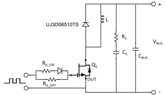
Figure 30. Schematic of the Chopper Mode Switching Test Circuit. Note, a Bus RC Snubber ( R_S = 2.5\text{ }\Omega , C_S = 100\text{ nF} ) is Used to Reduce the Power Loop High Frequency Oscillations.
