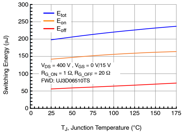
Figure 27. Clamped Inductive Switching Energy vs. Junction Temperature at V_{DS} = 400\text{ V} and I_D = 20\text{ A}
