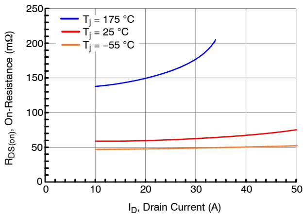
Figure 5. Typical Drain-Source On-Resistances at V_{GS} = 12\text{ V}
