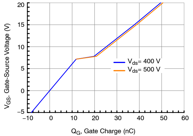
Figure 8. Typical Gate Charge at I_D = 20\text{ A}
