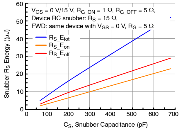
Figure 26. RC Snubber Energy Losses vs. Snubber Capacitance C_S at V_{DS} = 400\text{ V} , I_D = 25\text{ A} and T_J = 25\text{ °C}
