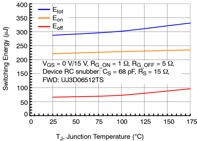
Figure 33. Clamped Inductive Switching Energy vs. Junction Temperature at V_{DS} = 400 \text{ V} and I_D = 25 \text{ A}
