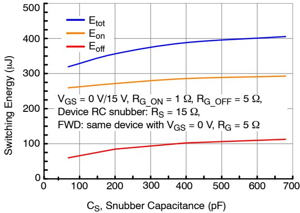
Figure 25. Clamped Inductive Switching Energies vs. Snubber Capacitance C_S at V_{DS} = 400\text{ V} , I_D = 25\text{ A} and T_J = 25\text{ °C}
