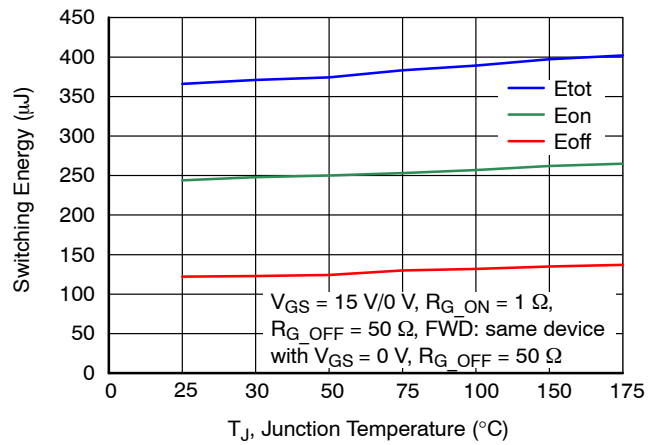
Figure 22. Clamped Inductive Switching Energy vs. Junction Temperature at V_{DS} = 400 V and I_D = 40 A
