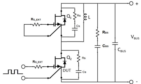
Figure 24. Schematic of the Half-bridge Mode Switching Test Circuit with Device RC Snubbers ( R_S = 10 Ω, C_S = 200 pF) and a Bus RC Snubber ( R_{BS} = 2.5 Ω, C_{BS} = 100 nF)
