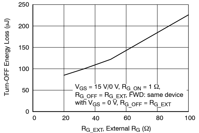
Figure 20. Clamped Inductive Switching Turn-off Energy vs. R_{G\_EXT} at V_{DS} = 400 V, I_D = 40 A, and T_J = 25 °C
