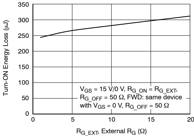
Figure 21. Clamped Inductive Switching Turn-on Energy vs. R_{G\_EXT} at V_{DS} = 400 V, I_D = 40 A, and T_J = 25 °C
