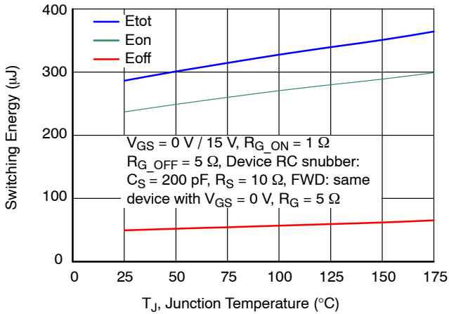
Figure 27. Clamped Inductive Switching Energy vs. Junction Temperature at V_{DS} = 400\text{ V} and I_D = 40\text{ A}
