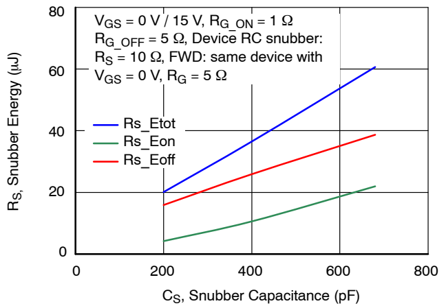
Figure 26. RC Snubber Energy Losses vs. Snubber Capacitance C_S at V_{DS} = 400\text{ V} , I_D = 40\text{ A} , and T_J = 25\text{ °C}
