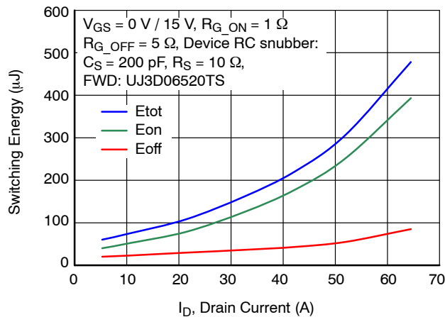
Figure 29. Clamped Inductive Switching Energies vs. Drain Current at V_{DS} = 400\text{ V} and T_J = 25\text{ °C}
