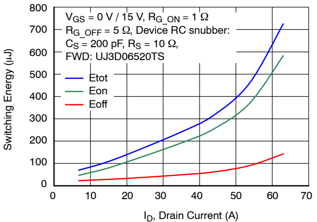
Figure 30. Clamped Inductive Switching Energies vs. Drain Current at V_{DS} = 500\text{ V} and T_J = 25\text{ °C}
