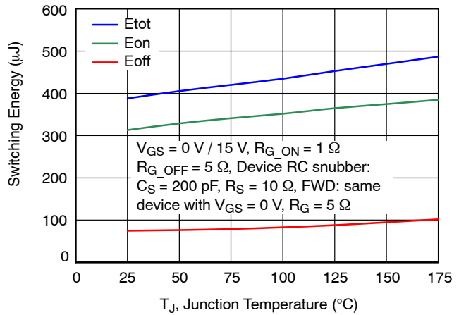
Figure 28. Clamped Inductive Switching Energy vs. Junction Temperature at V_{DS} = 500\text{ V} and I_D = 40\text{ A}
