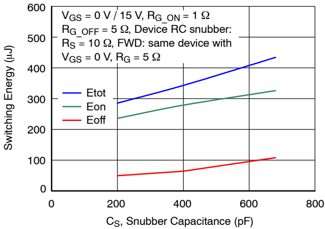
Figure 25. Clamped Inductive Switching Energy vs. Snubber Capacitance C_S at V_{DS} = 400\text{ V} , I_D = 40\text{ A} and T_J = 25\text{ °C}
