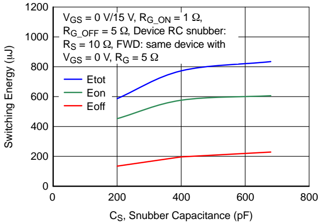
Figure 25. Clamped Inductive Switching Energies vs. Snubber Capacitance C_S at V_{DS} = 400\text{ V} , I_D = 40\text{ A} and T_J = 25\text{ °C}
