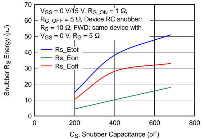
Figure 26. RC Snubber Energy Losses vs. Snubber Capacitance C_S at V_{DS} = 400\text{ V} , I_D = 40\text{ A} and T_J = 25\text{ °C}
