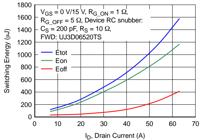
Figure 30. Clamped Inductive Switching Energy vs. Drain Current at V_{DS} = 500\text{ V} and T_J = 25\text{ °C}
