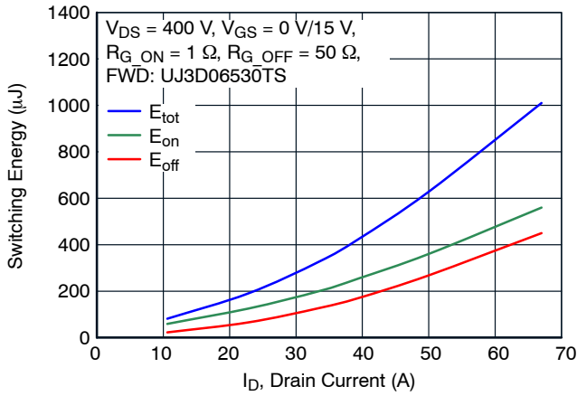
Figure 25. Clamped Inductive Switching Energy vs. Drain Current at V_{DS} = 400\text{ V} and T_J = 25\text{ }^\circ\text{C}
