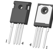
TO247-4 15.90x20.96x5.03, 5.44P CASE 340AN
