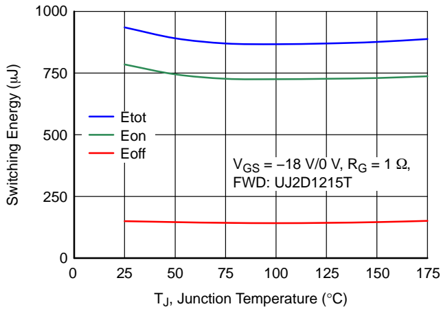
Figure 19. Clamped Inductive Switching Energy vs. Junction Temperature at V_{DS} = 800\text{ V} and I_D = 25\text{ A}
