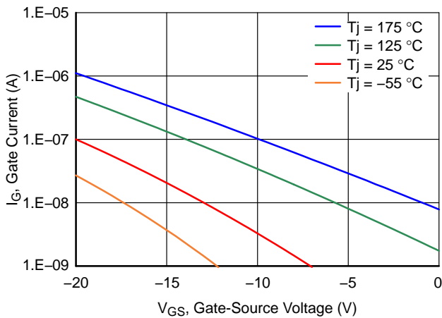
Figure 11. Typical Gate Leakage at V_{DS} = 0\text{ V}
