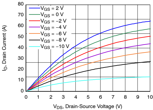
Figure 3. Typical Output Characteristics at T_J = 175\text{ }^\circ\text{C}
