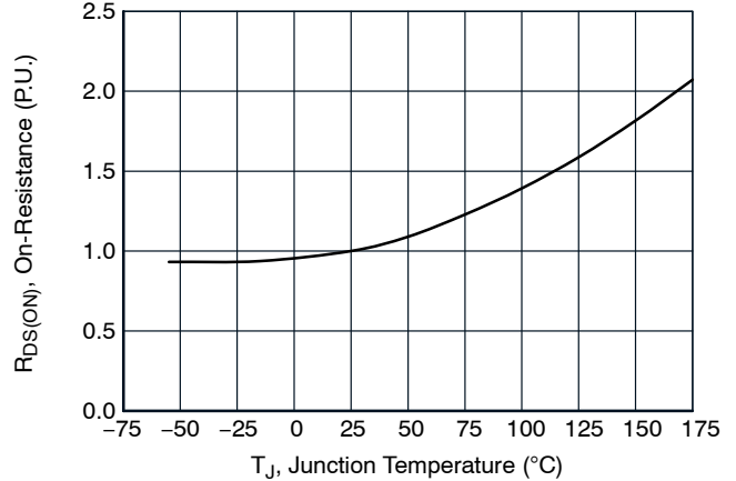
Figure 4. Normalized On-Resistance vs. Temperature at V_{GS} = 12\text{ V} and I_D = 40\text{ A}
