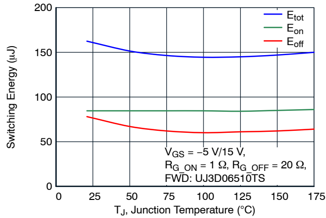
Figure 21. Clamped Inductive Switching Energy vs. Junction Temperature at V_{DS} = 400\text{ V} and I_D = 20\text{ A}
